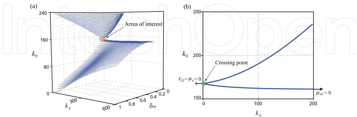
Figure 5. (a) A set of dispersion curves of the TE bulk polaritons for different filling factors \delta_m for the structure being in the Voigt geometry and (b) manifestation of crossing effect in dispersion curves of the TE bulk polaritons at the particular value of filling factor \delta_m = 0.132 . Parameters of magnetic constitutive layers are shown in Figure 2 . For the semiconductor constitutive layers, parameters are f_p = \omega_p/2\pi = 10.5 GHz, f_c = \omega_c/2\pi = 9.5 GHz, \nu = 0 , \varepsilon_l = 1.0 , and \mu_s = 1.0 .
