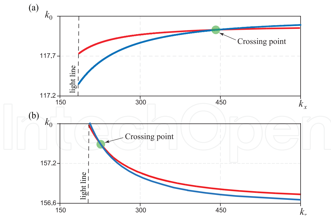
Figure 8. Manifestation of the crossing effect in dispersion curves of hybrid EH (red line) and HE (blue line) surface polaritons; (a) polar configuration ( \delta_m = 0.27 ) and (b) Faraday configuration ( \delta_m = 0.15 ). All structure constitutive parameters are shown in Figure 2 .
