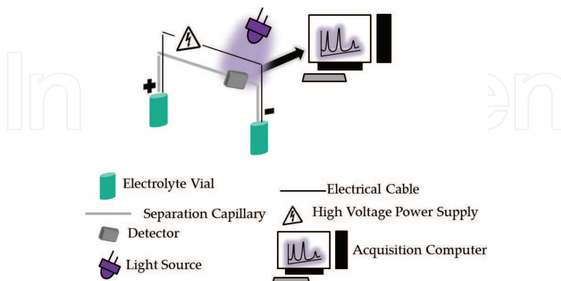
Figure 1. Scheme of CE setup.
