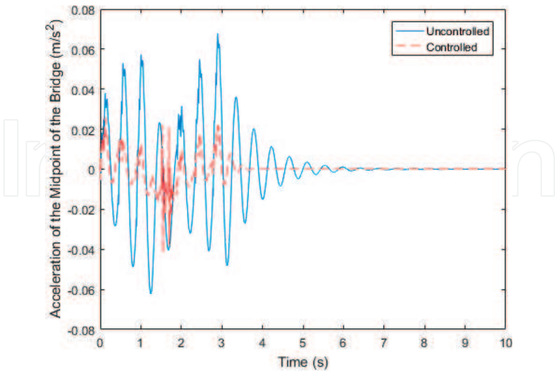
Figure 7. Acceleration of the midpoint of the railway bridge.
