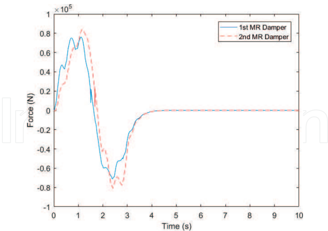
Figure 8. Two MR dampers' forces.
