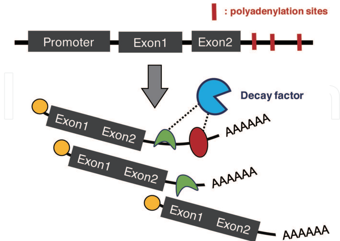
Figure 3. Alternative polyadenylation affects 3'UTR lengths. Longer UTRs allow more RBPs to associate with the mRNA (indicated by arrowhead and ellipse, respectively). The RBPs regulate the mRNA stability by recruiting decay factor.
