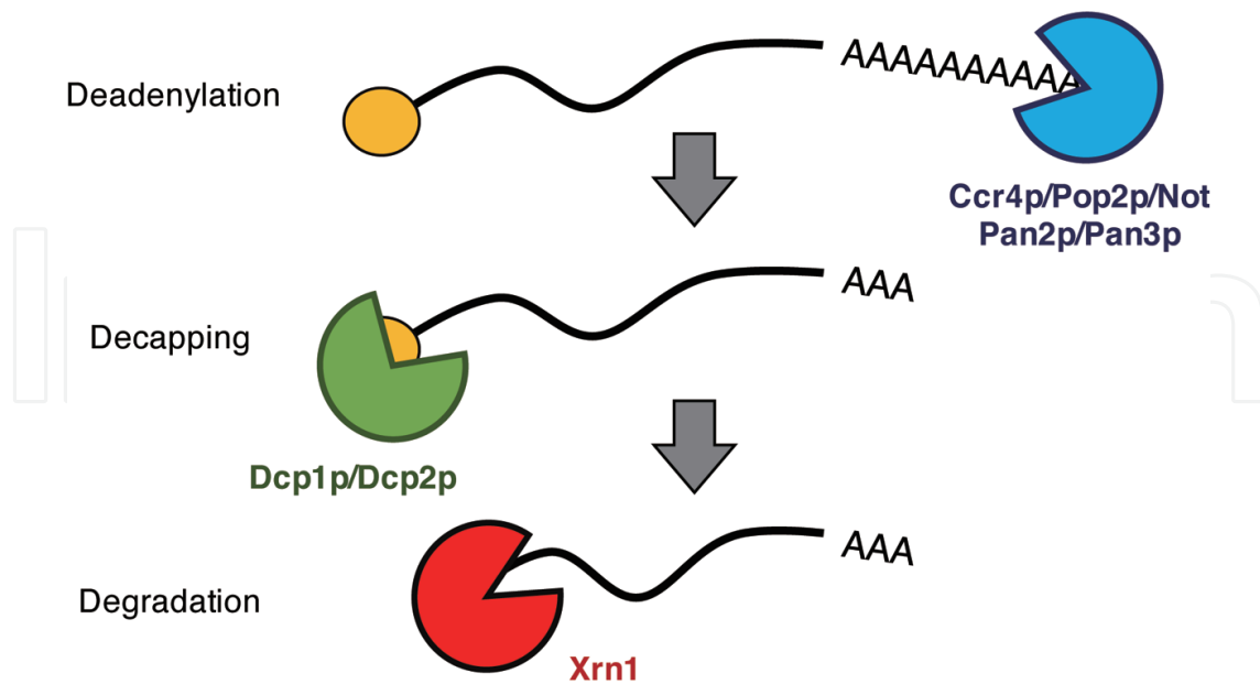
Figure 2. The 5' → 3' degradation pathway exonuclease-mediated decay begins with shortening of Pan2/Pan3 or CCR4-not complexes. After the decapping of 5'cap structure (a circle), the body of mRNA is degraded with 5'-to-3'polarity by XRN1.
