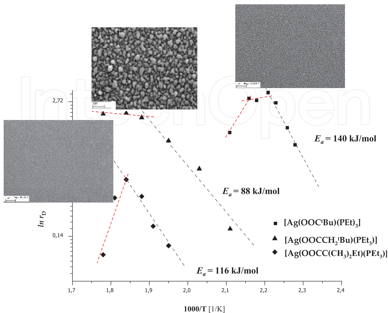
Figure 2. Influence of the carboxyl are groups on the morphology of silver layers, the deposition rate, and the value of activation energies (CVD technique, precursor [\text{Ag}(\text{OOCR}')(\text{PEt}_3)] ; \text{R}' = -^t\text{Bu} (a), -\text{CH}_2^t\text{Bu} (b), and -\text{C}(\text{Me}_2)\text{et} (c)).
