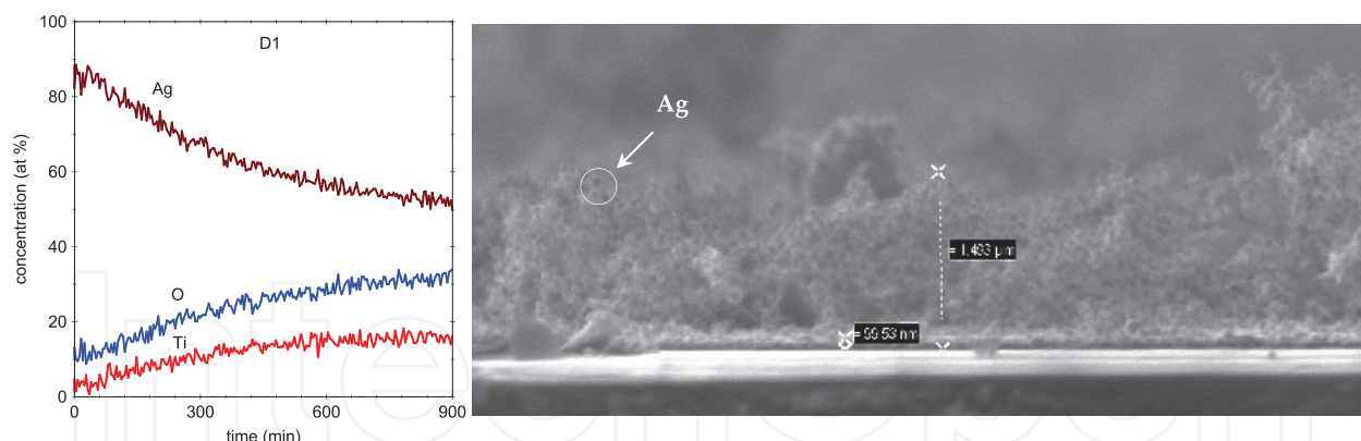
Figure 6. SEM images and XPS depth profile of the TiO 2 /Ag composite coating deposited on the surface of titanium implant (CVD, titania matrix were obtained using [Ti 6 O 6 (H 2 O) 2 (O i Bu) 6 (OOC i Bu) 6 ] as the precursor, T_D = 713 K, p = 3 hPa, t = 60 min, Ar, and silver nanoparticles were deposited using [Ag(OOCCH 2 i Bu)(PEt 3 )] as the precursor, T_D = 433 K, p = 1.5 hPa, t = 60 min, Ar) [52].
