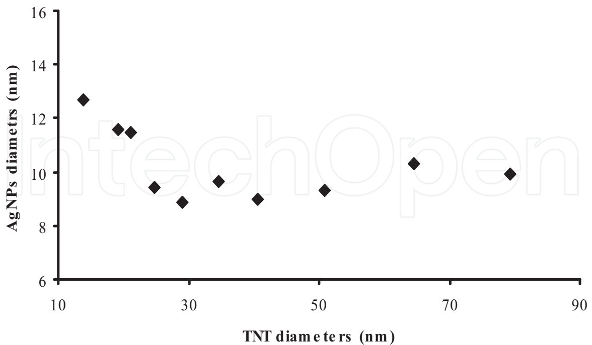
Figure 4. Effect of TNT surface morphology on the diameter of AgNPs after 100 ALD cycles on the surface of Ti6Al4V/TNT substrates.
