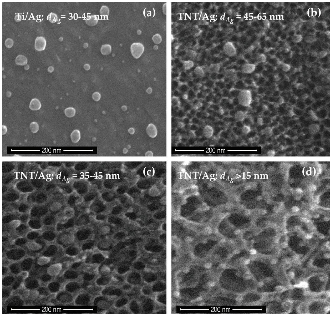
Figure 1. Scanning electron microscopy (SEM) images of titania nanotube coatings enriched with silver particles deposited by CVD method ((a) reference sample, (b) d_{TNT} = 23-30 nm, (c) d_{TNT} = 30-45 nm, (d) d_{TNT} = 80-150 nm) [46].
