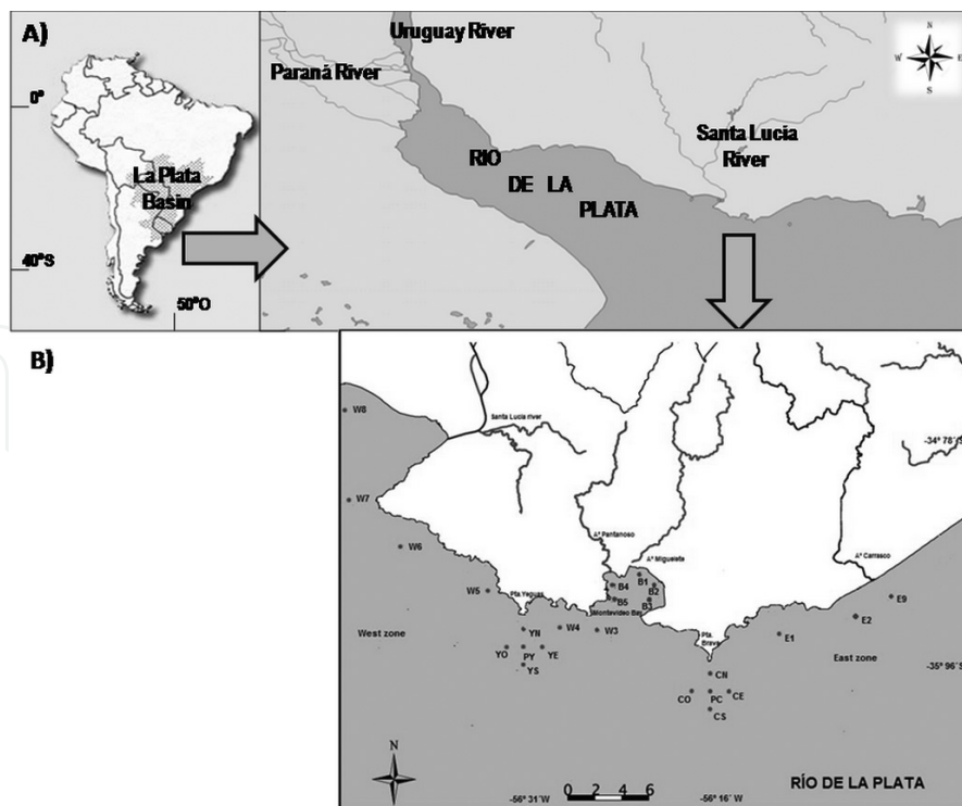
Figure 1. Location of the La Plata Basin, RdIP and Montevideo coastal zone (MCZ) with Punta Brava and sampling sites.
