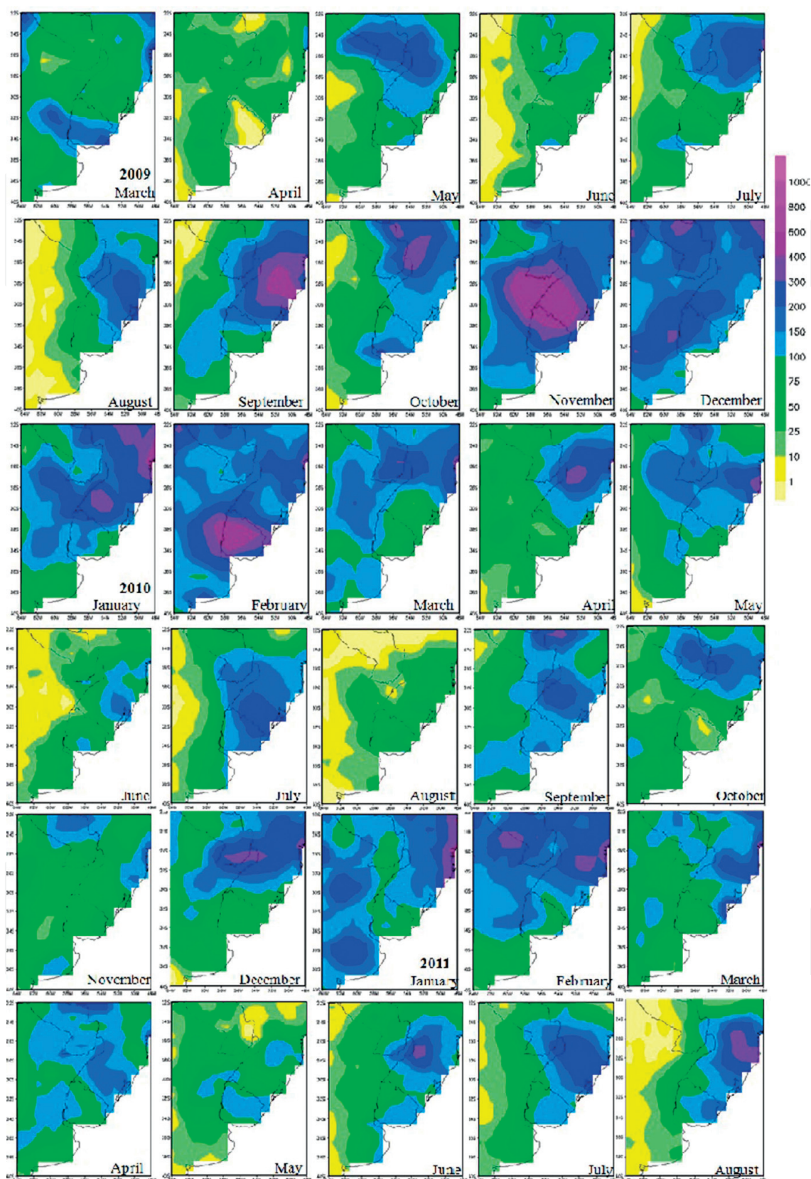
Figure 3. Total monthly precipitation (mm month -1 ) on the surface of the earth to the region 22°00'–40°00' S and 48°00'–64°00' W.
