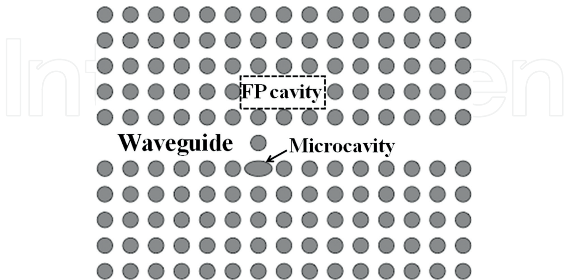
Figure 17. Optical diode based on asymmetrical coupling by a microcavity and FP cavity at two sides of PhC waveguide [39].
