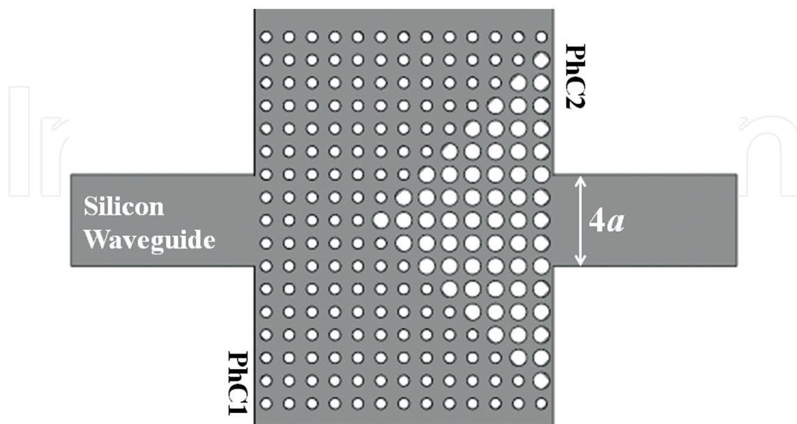
Figure 13. Optical diode with PhC heterostructure connecting standard silicon waveguide [29].
