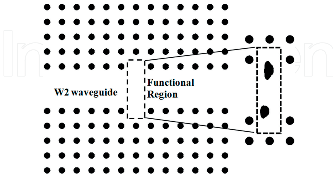
Figure 10. The broadband optical diode in PhC waveguide with 4 \times 1 unit cells' compact-optimized functional region [26].
