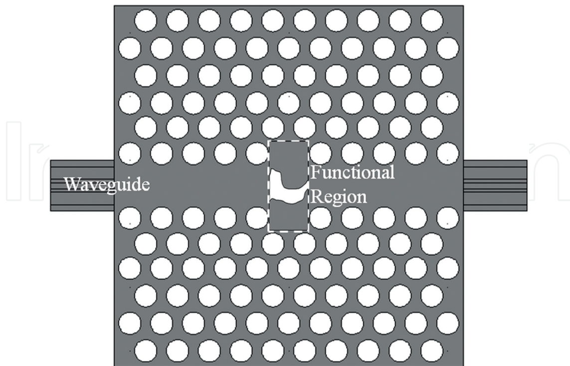
Figure 14. Optical diode with topological optimized functional region connecting silicon waveguide [32].
