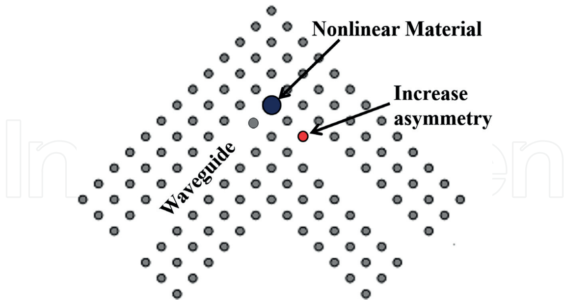
Figure 16. Optical diode based on dipole modes of Kerr microcavity in asymmetric L-shaped PhC waveguide [38].
