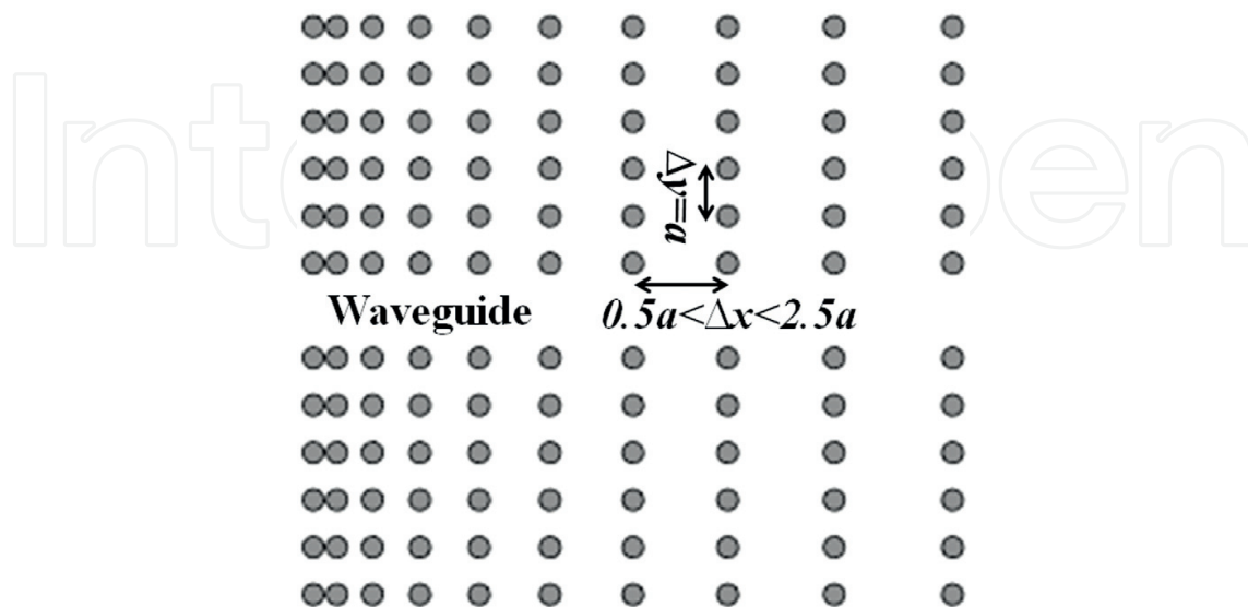
Figure 6. The optical diode in PhC waveguide with chirped PhC structure [19].
