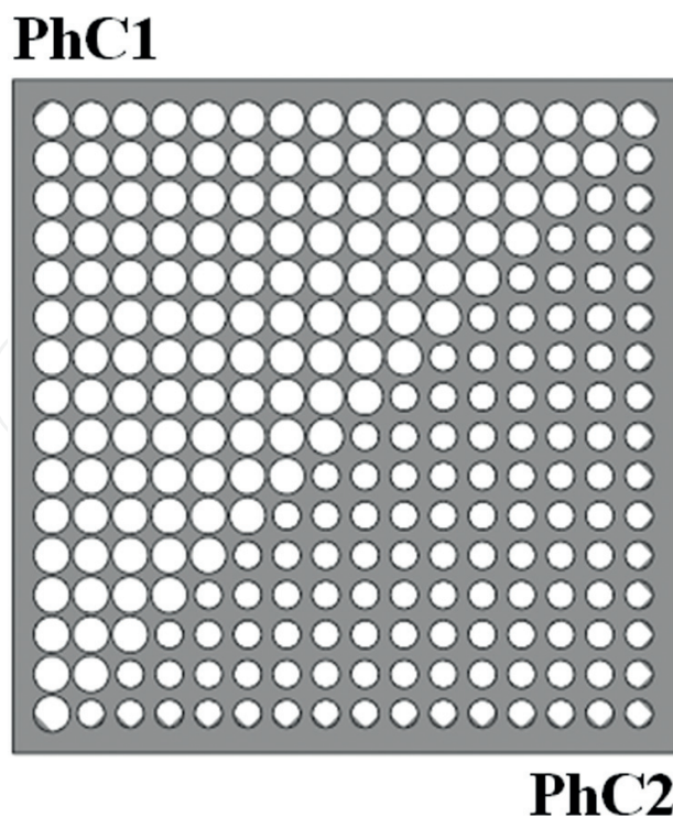
Figure 12. Refraction-based optical diode with PhC heterostructure [31].
