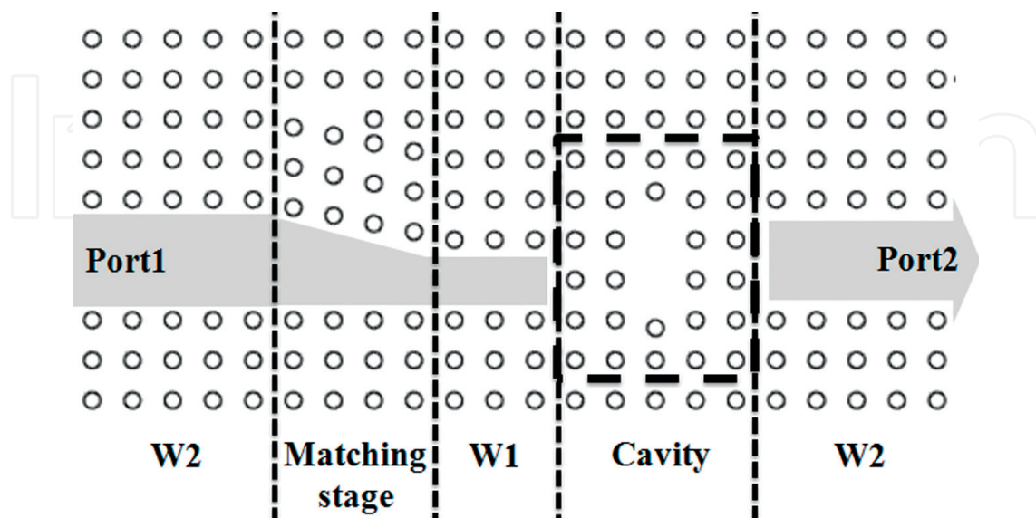
Figure 3. Coupling structure consists of PhC waveguides with the cavity [16].
