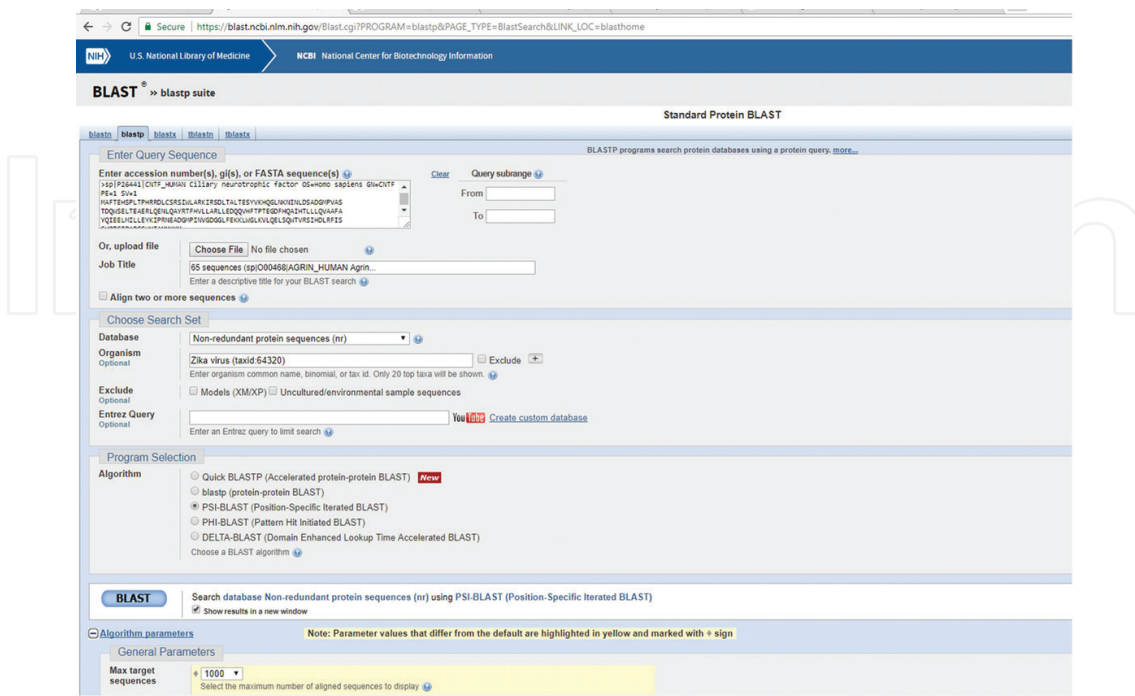
Figure 9. BLAST search.
