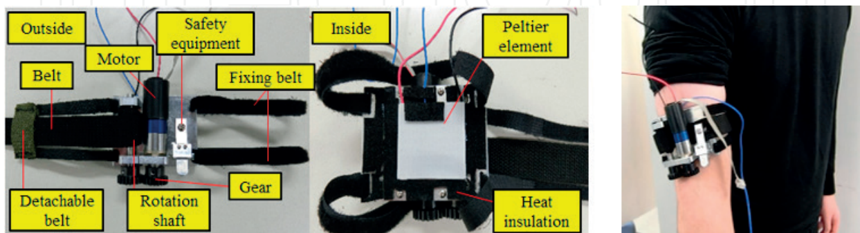
Figure 10. Two-sensory feedback device and its attached state.
