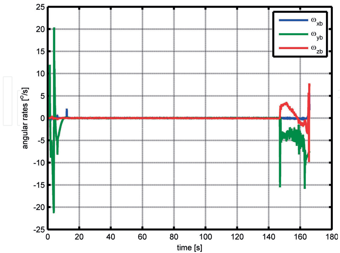
Figure 9. Input data from gyroscopes used for simulation.
