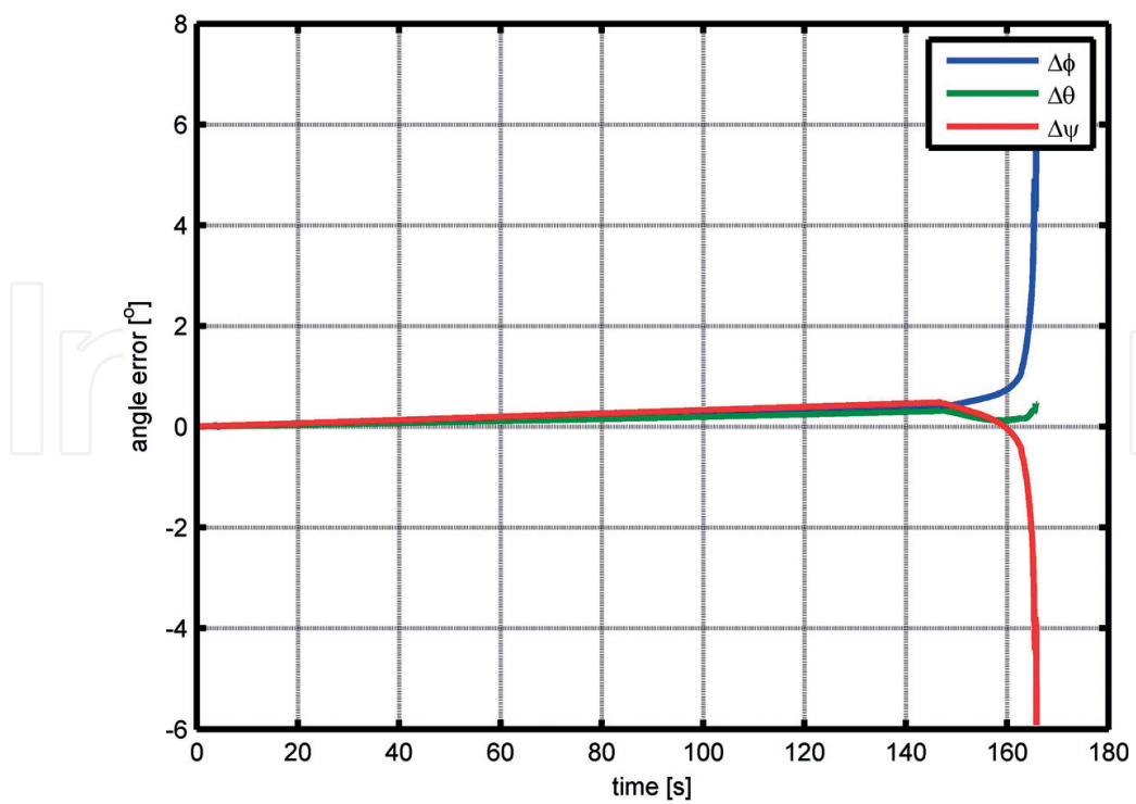
Figure 10. Angle error accumulation in time.
