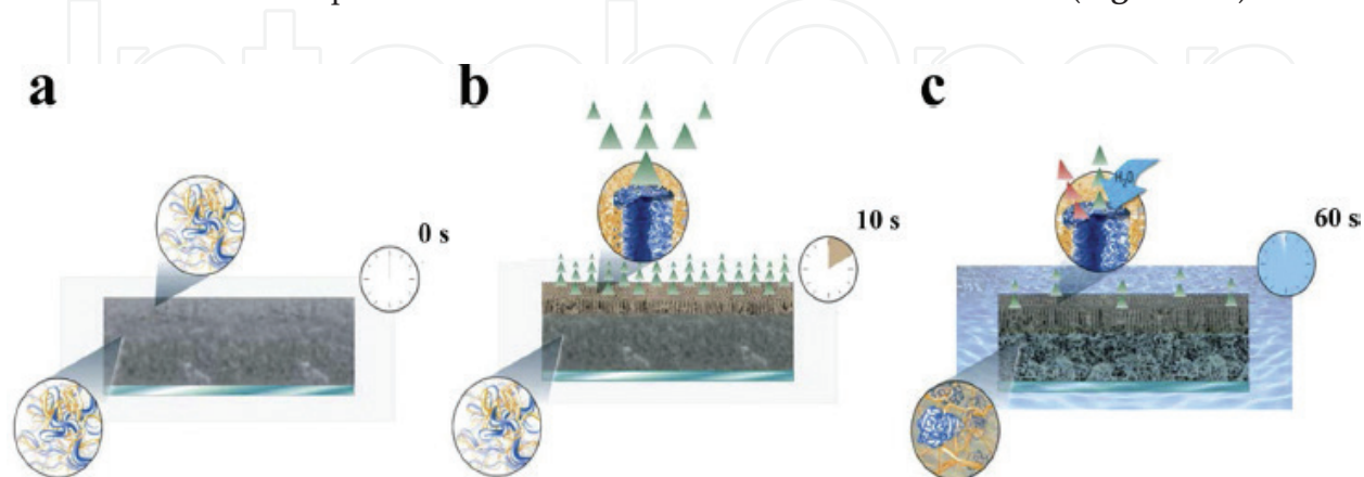
Figure 32. Schematic diagram of the asymmetric film formation process combining NIPS with the self-assembly of block copolymer PS- b -P4VP. Source: Ref. [152], Copyright 2007; reproduced with permission from the Nature Publishing Group.
