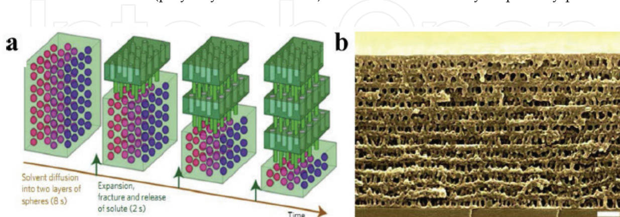
Figure 33. (a) Schematic of the osmotic shock process acting on layers of spheres and leading to the perforated multi layers. (b) Fracture cross-section of PS- b -PMMA multilayer structures (scale bar, 200 nm). Source: Ref. [155], Copyright 2012; reproduced with permission from the Nature Publishing Group.
