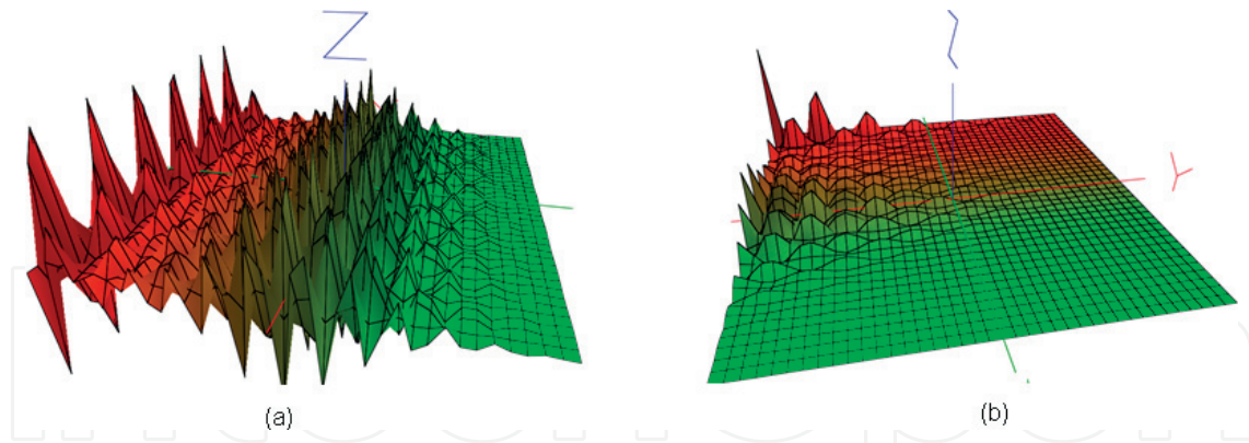
Figure 1. (a) Model of space-time with matter production without Immirzi parameter, but yes torsion. (b) Model of space-time with gravity and Immirzi parameter, including torsion. Observe the non-symmetric space created in the waving movement due to gravity.
