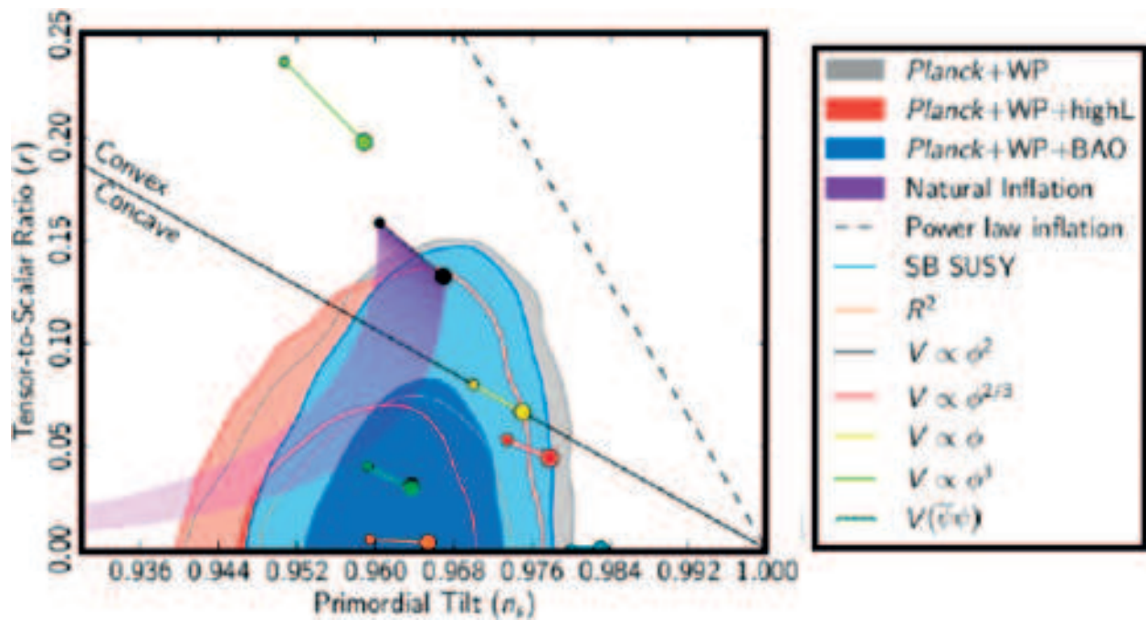
Figure 3. Energy-matter tensor development in the lepto-genesis and baryon-genesis processes. The SB SUSY region or area is where takes form the space U_7^S . the convexity in the thermal and expansion arrow meets to the causal structure of the universe defined by the light cones and given by the homomorphism (15).
