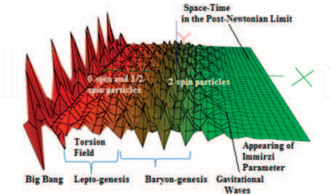
Figure 2. Evolution of the Universe and gravitational sequence of the energy-matter tensor [9, 12–14].
