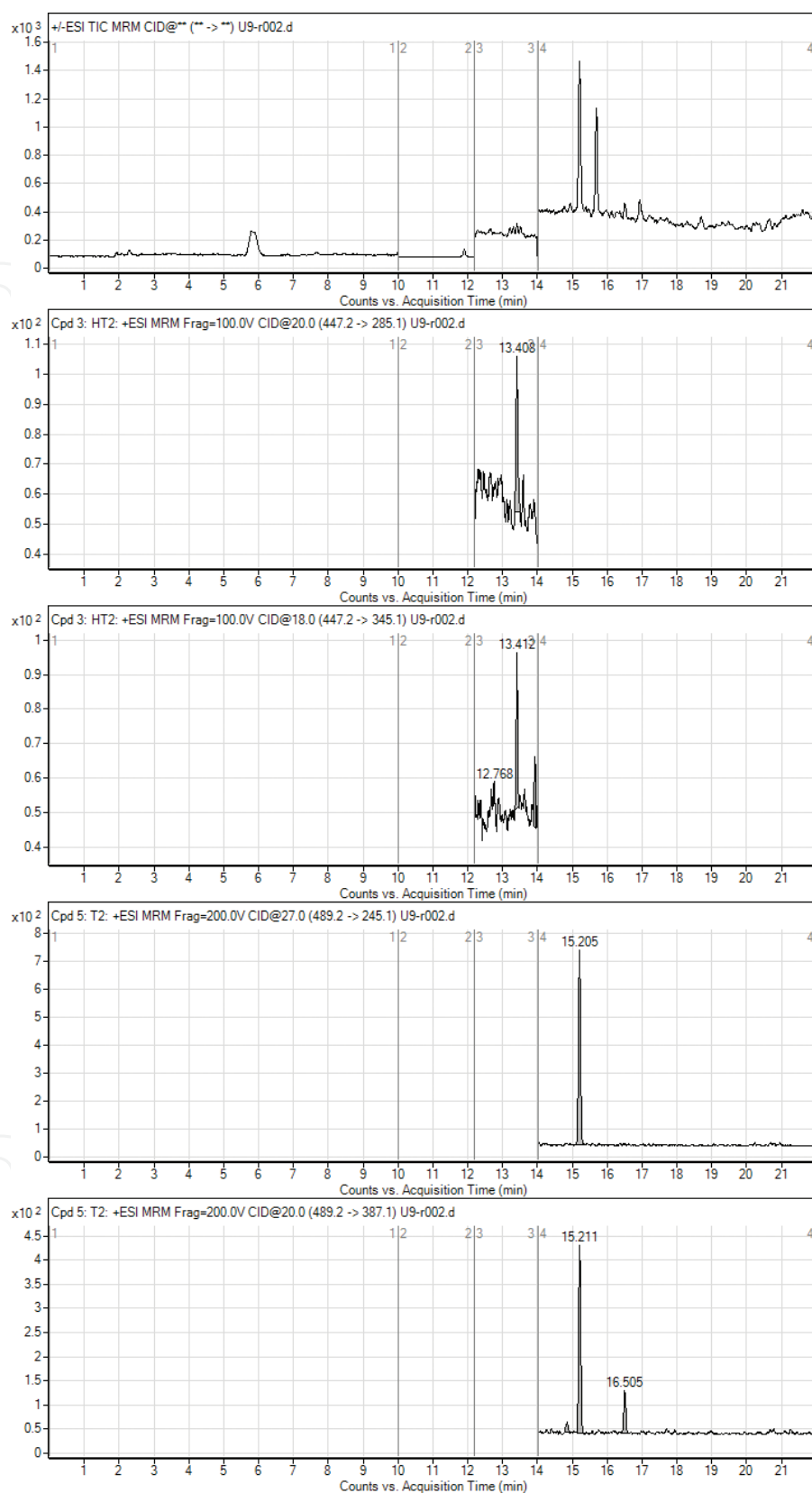
Figure 3. A typical LC-MS/MS-MRM chromatogram of a contaminated maize sample after roasting at the temperature of 220°C for 30 min (50.3 \mu\text{g}/\text{kg} of T-2 and 138 \mu\text{g}/\text{kg} of HT-2); TIC; HT-2 MRM 447.2 \rightarrow 285.1; HT-2 MRM 447.2 \rightarrow 345.1; T-2 MRM 489.2 \rightarrow 245.1; and T-2 MRM 489.2 \rightarrow 387.1.
