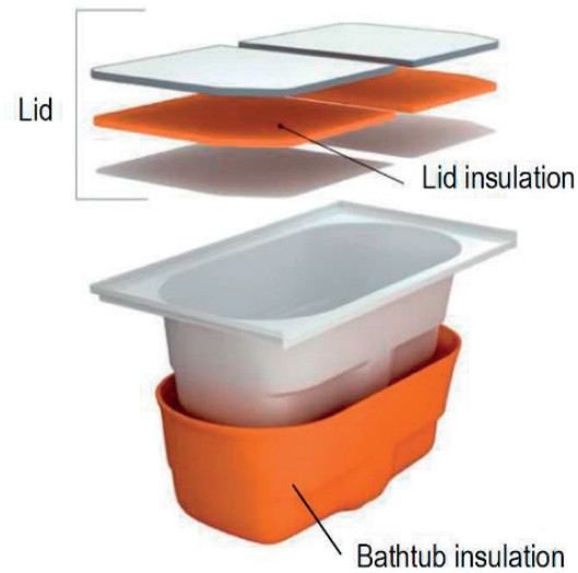
Structure of the insulated bathtub
