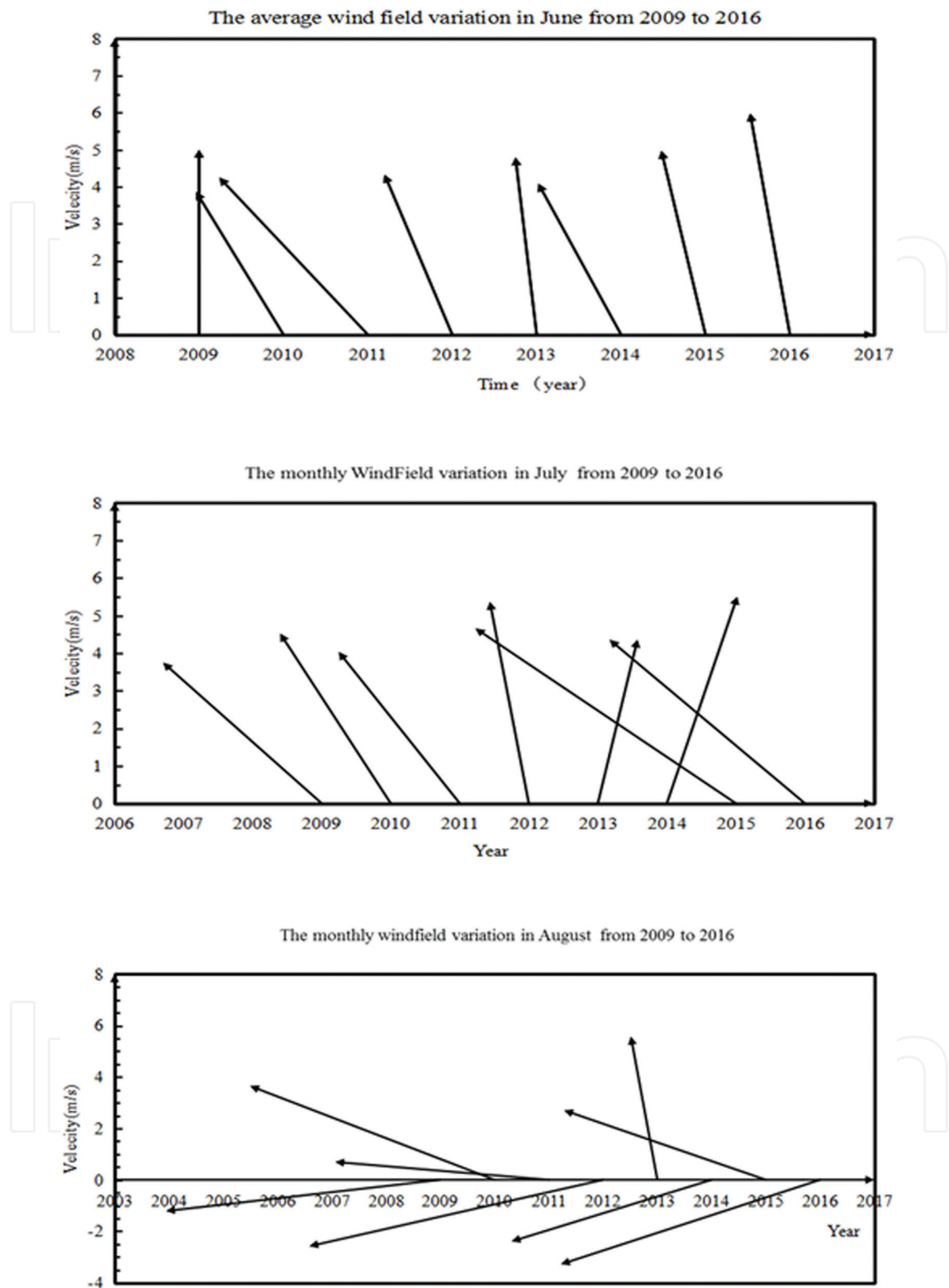
Figure 4. Average wind field variation in Qianliyan area in June (a), July (b), and August (c) 2009–2016.
