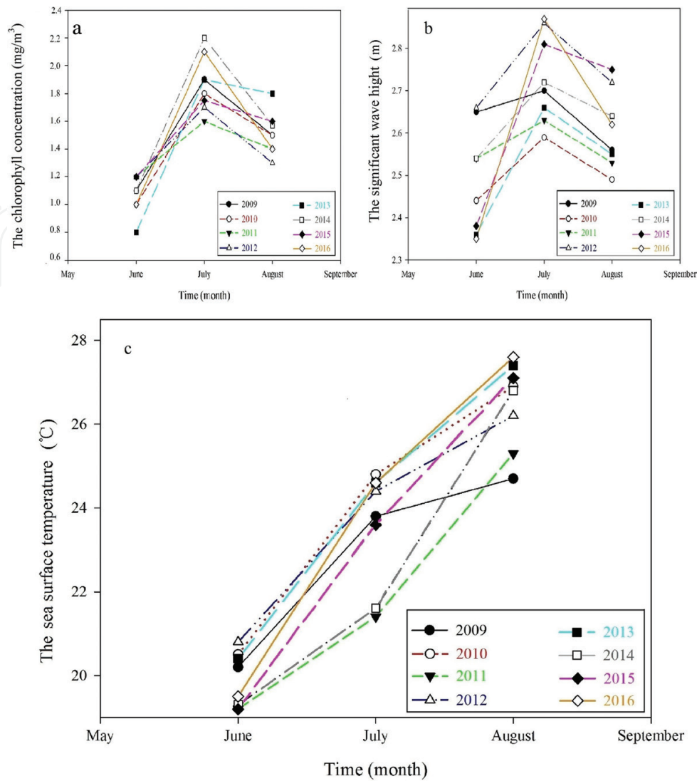
Figure 2. Average CHL (a), SWH (b), and SST (c) in June, July, and August, respectively from 2009 to 2016.
