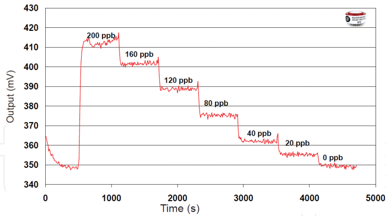
Figure 4. Response to 200 ppb SO 2 using the SO 2 sensor.
