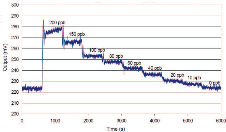
Figure 6. Response to 200 ppb O 3 using the O 3 sensor.
