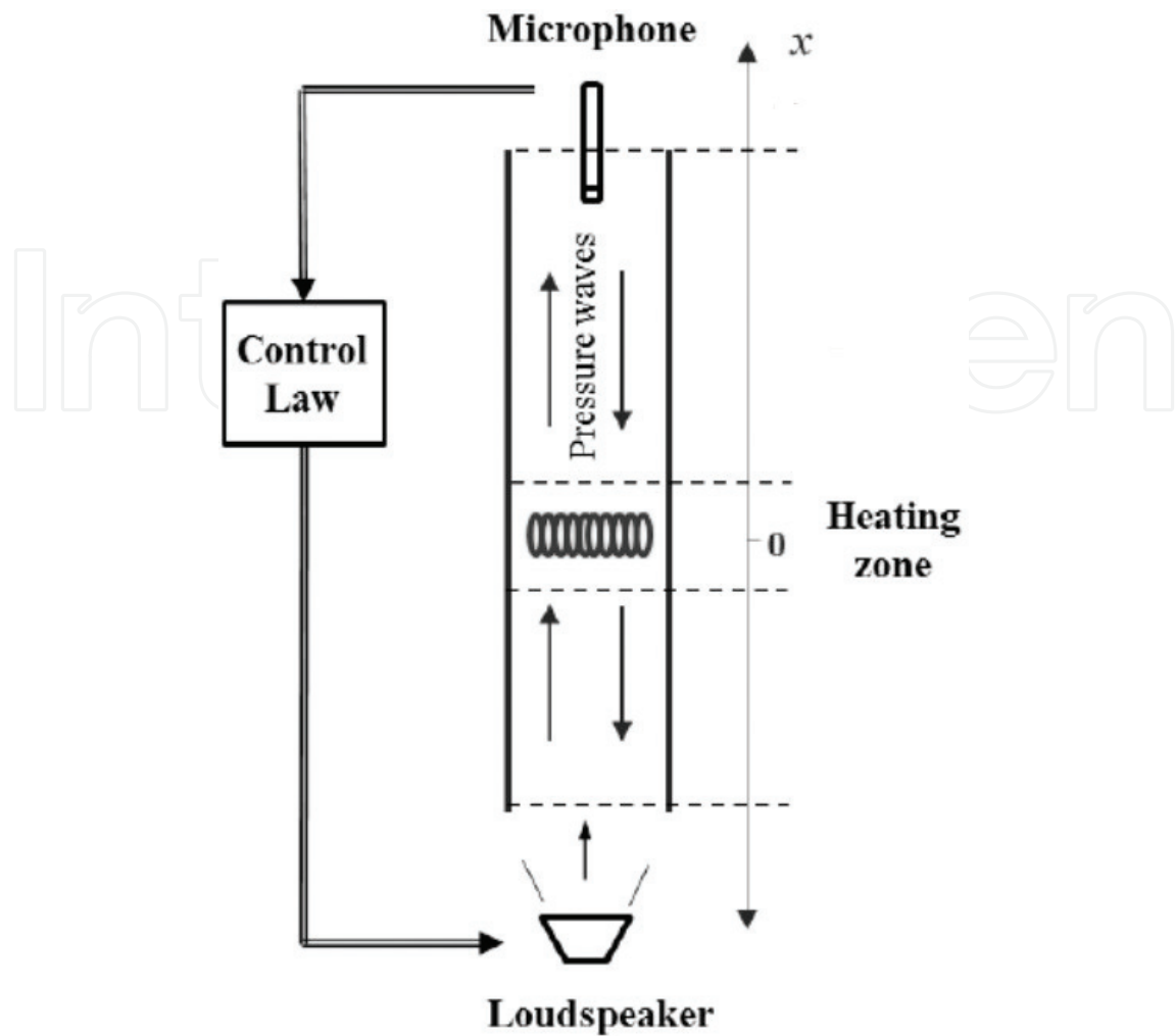
Figure 1. A functional implementation diagram of a thermoacoustic oscillation control system, including a microphone for sensing and a loudspeaker for actuation.
