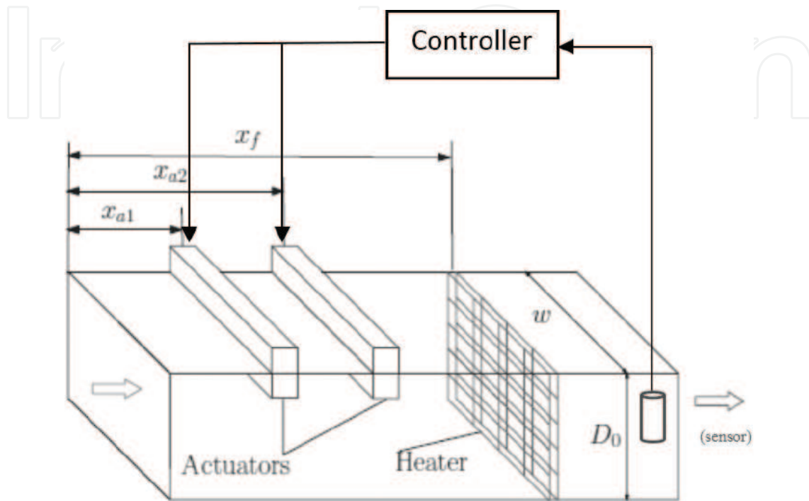
Figure 2. A control-oriented schematic of a combustion system with actuators modeled as monopole-like moving pistons.
