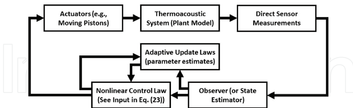
Figure 3. A block diagram illustrating the main components of the proposed robust and adaptive thermoacoustic oscillation control system.
