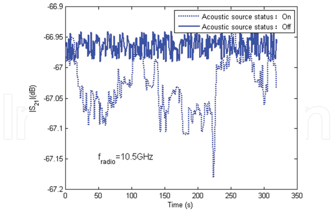
Figure 13. The testing result of 10.5 GHz stimulated by the “double-slit” acoustic source.
