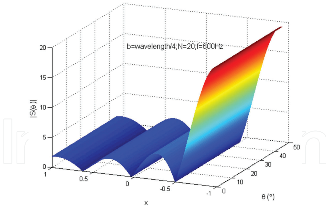
Figure 8. The simulation example of the array factor of the acoustic antenna array in Figure 6.
