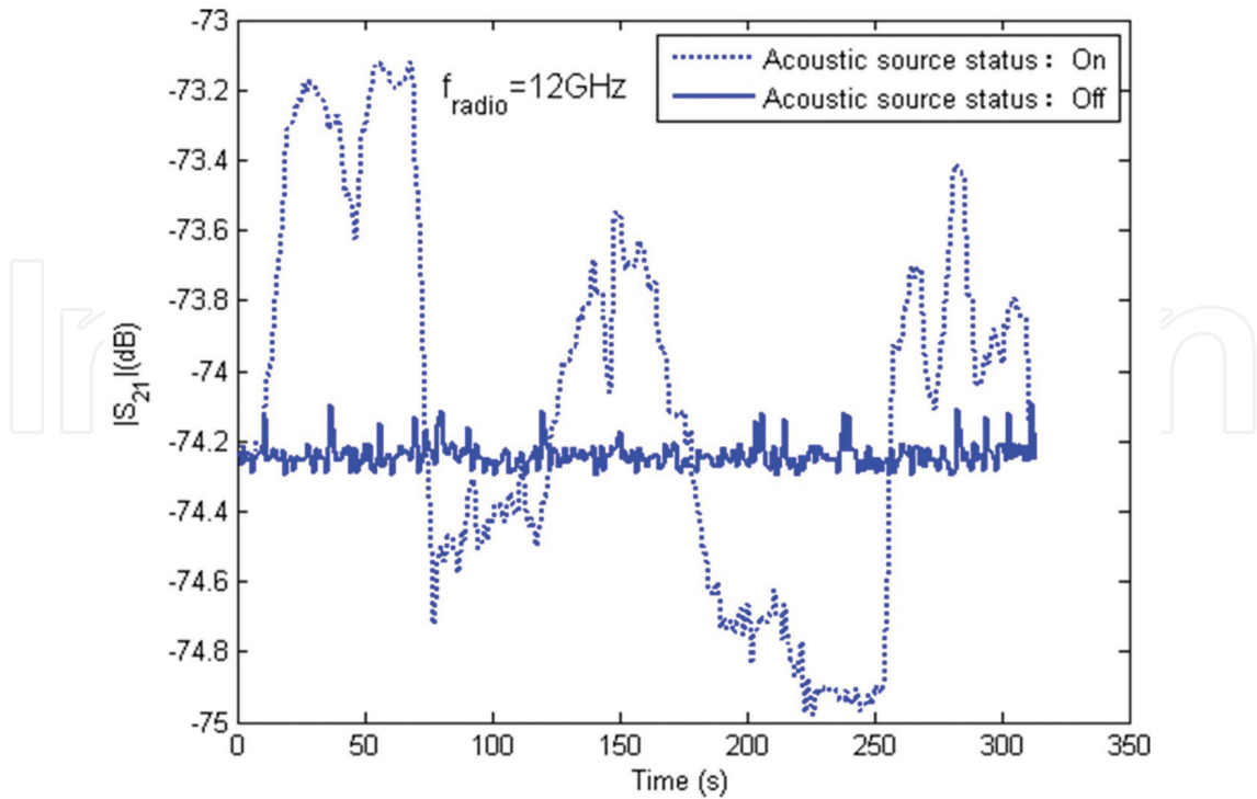
Figure 18. The testing result of 12 GHz stimulated by the “7 × 7 hole” acoustic source.
