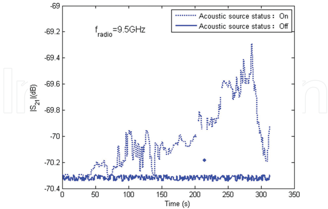
Figure 16. The testing result of 9.5 GHz stimulated by the “7 × 7 hole” acoustic source.
