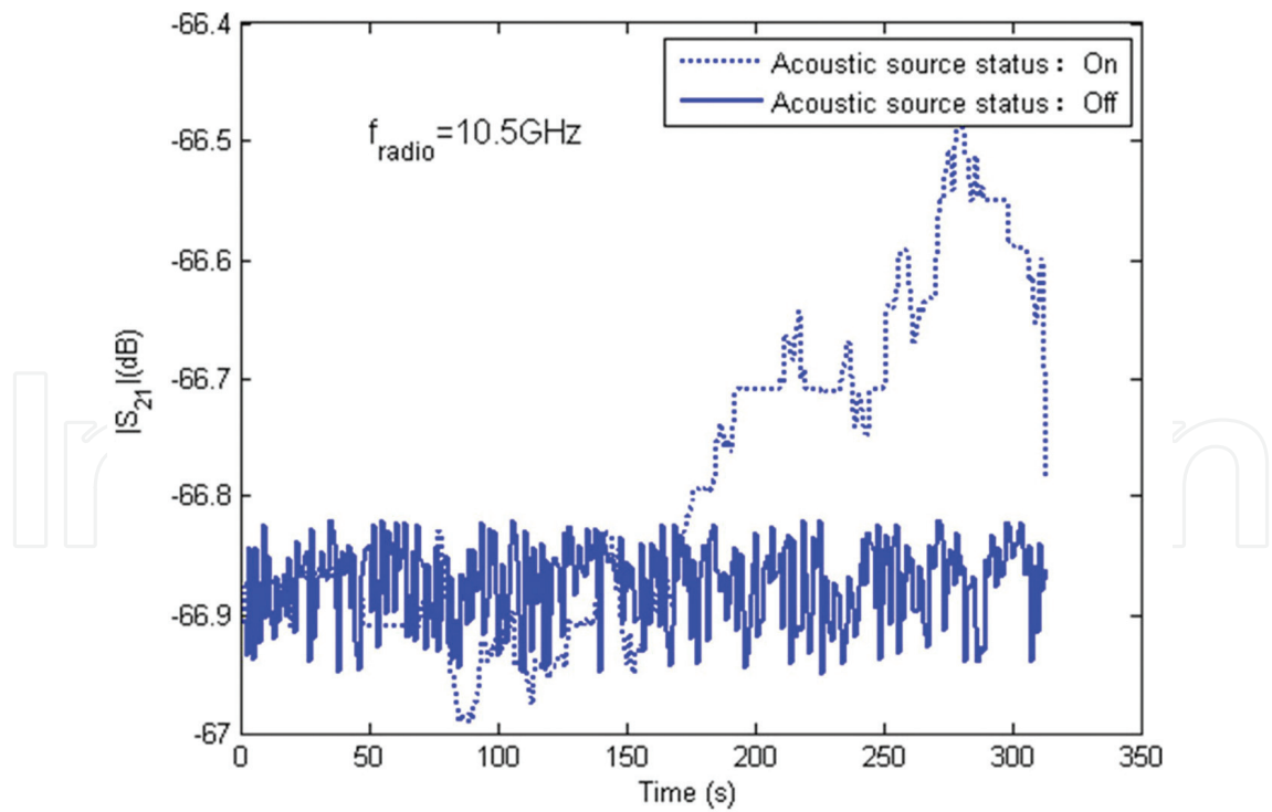
Figure 17. The testing result of 10.5 GHz stimulated by the “7 × 7 hole” acoustic source.
