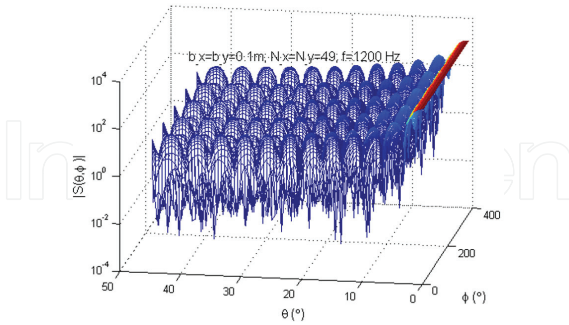
Figure 7. The simulation example of the array factor of the acoustic antenna array in Figure 5.
