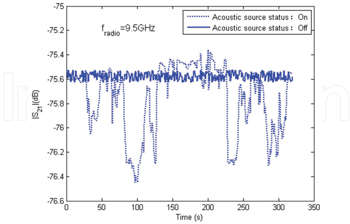
Figure 12. The testing result of 9.5 GHz stimulated by the “double-slit” acoustic source.
