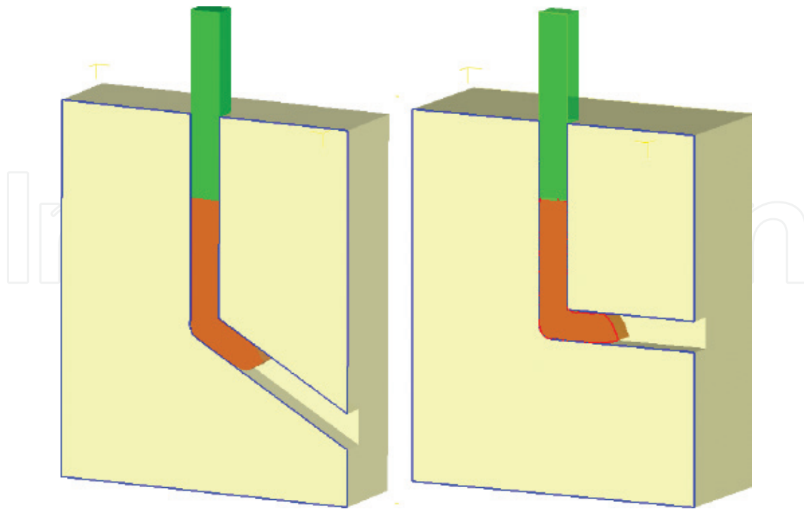
Figure 2. ECAP principles (channel intersecting at 120° and 90°, respectively) [10].
