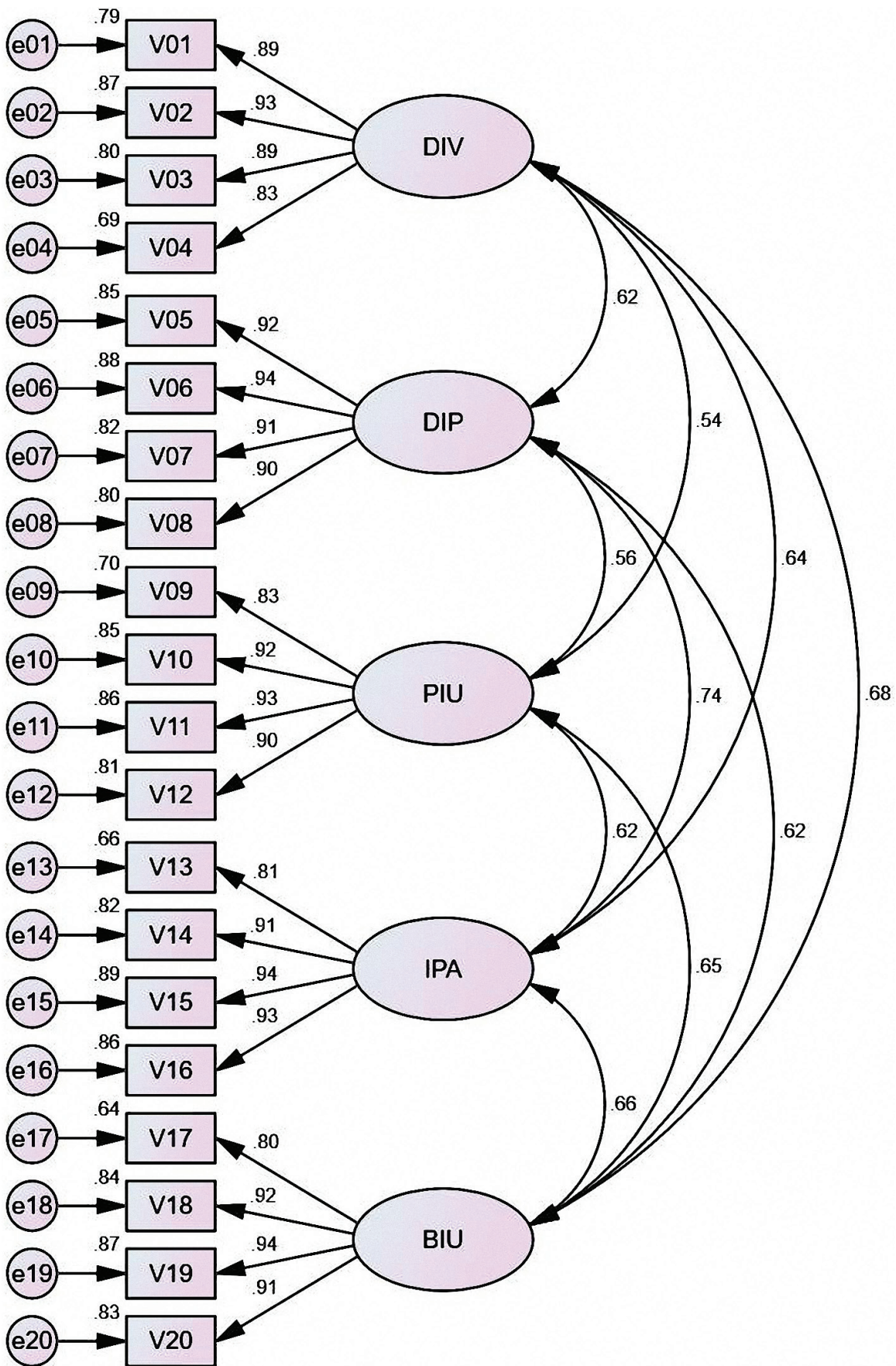
Figure 2. Measurement model.
