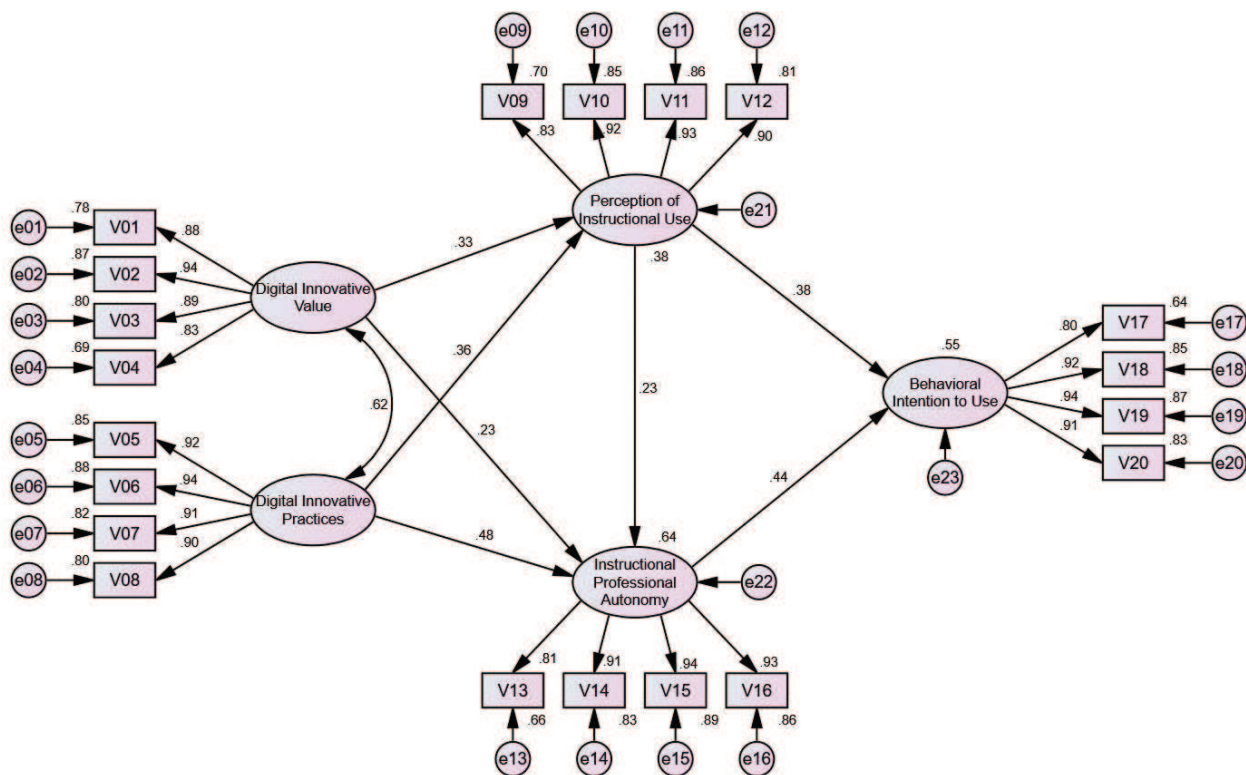
Figure 3. Structural model.
