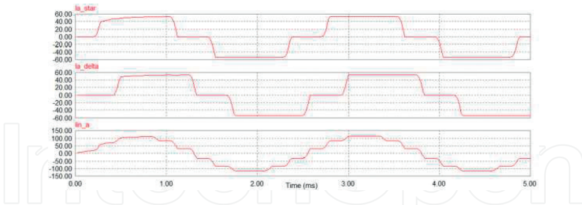
Figure 4. Current waveforms for phase (a) at input frequency 400 Hz.
