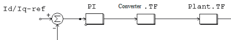
Figure 13. Close loop control of inner current control. PI TF: K_p + K_i \frac{1}{s} = K_p \left( \frac{s + a_i}{s} \right) ; converter TF: \frac{1}{1 + T_s s} ; plant TF: \frac{1}{R + Ls} .
