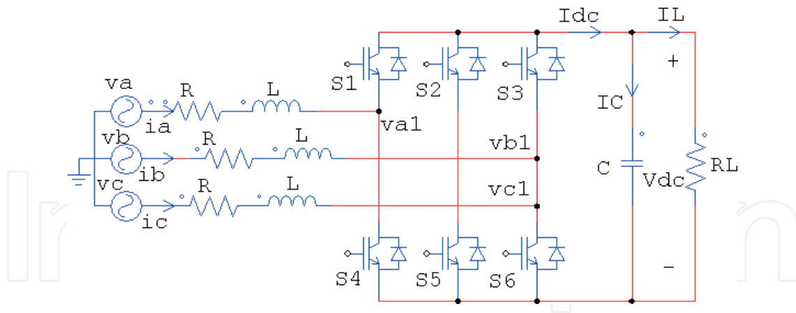
Figure 7. 6-pulse active rectifier configuration.
