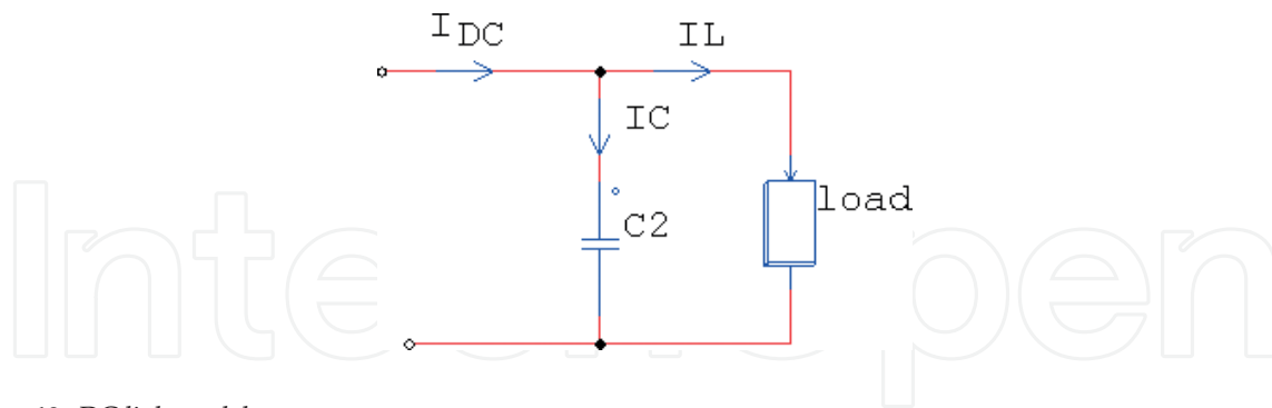
Figure 10. DC link model.
