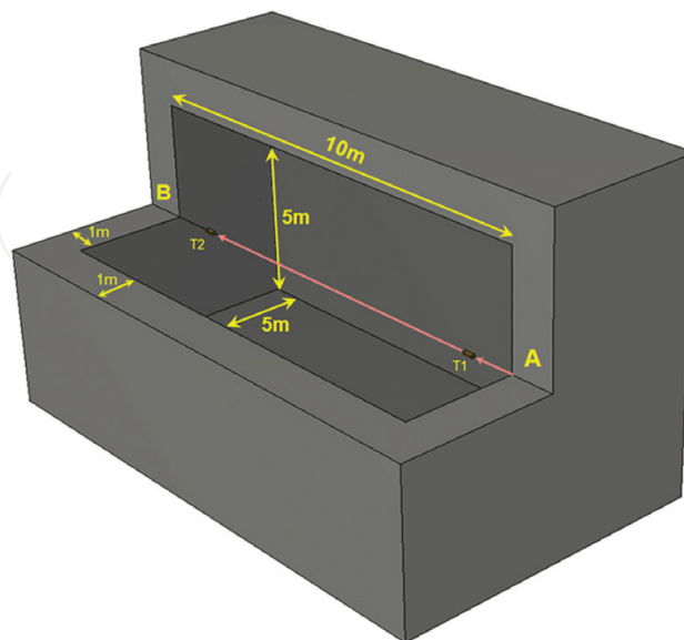
Figure 9. Generic model of accelerator hall.
