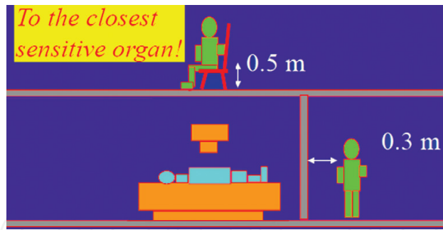
Figure 3. Dose evaluation points recommended by NCRP 147.
