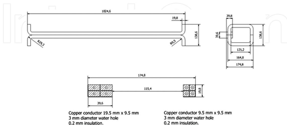
Figure 15. Thick magnetic extraction septum.
