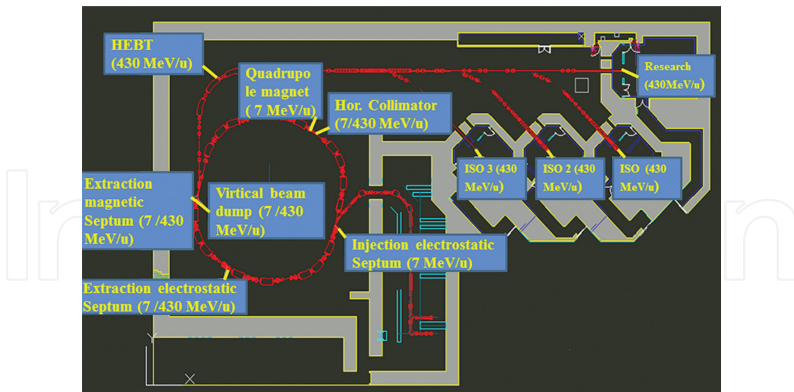
Figure 2. Graphical overview of beam loss points and four irradiation rooms. Typical energies at each loss point are shown.
