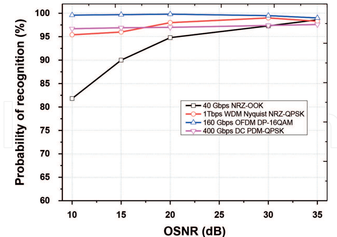
Figure 12. Percentage recognition versus OSNR values for NRZ-OOK, OFDM DP-16QAM, DC PDM-QPSK and WDM-Nyquist NRZ-DP-QPSK modulation types.
