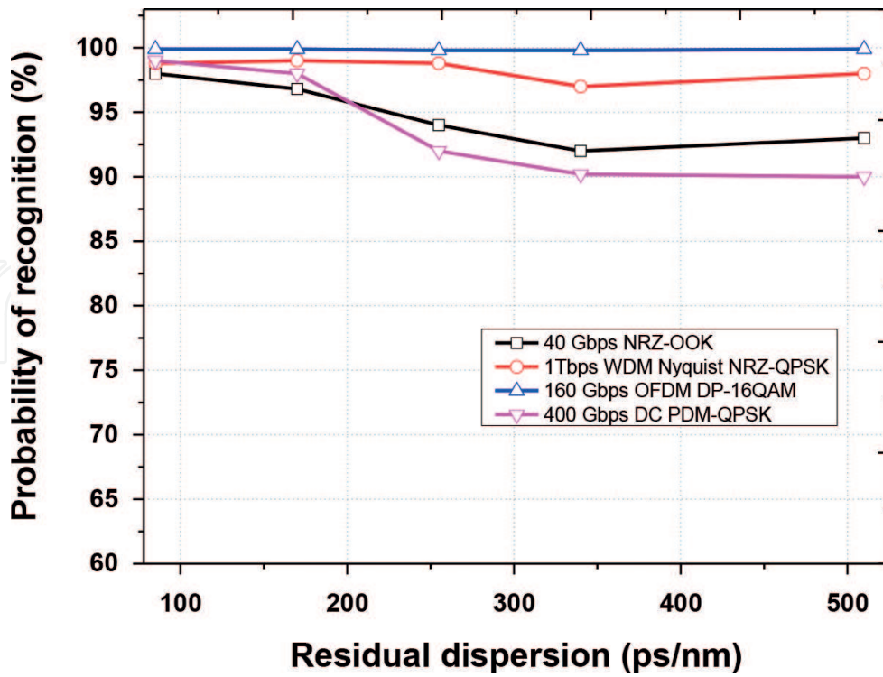
Figure 13. Percentage of correct identification for four used modulation formats depending upon residual dispersion for OSNR = 20 dB.
