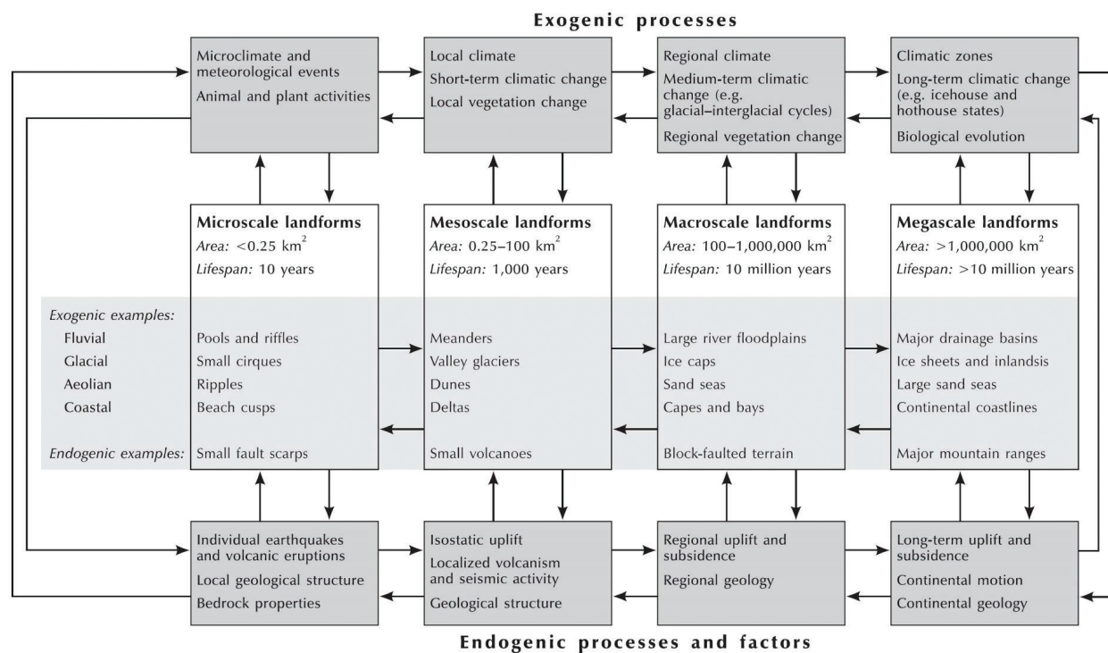
Figure 1. Form, process, and their interrelationships for the evolution of various landforms developed due to endogenic and exogenic processes over various scales of time and climatic zones (adapted from [6]).
