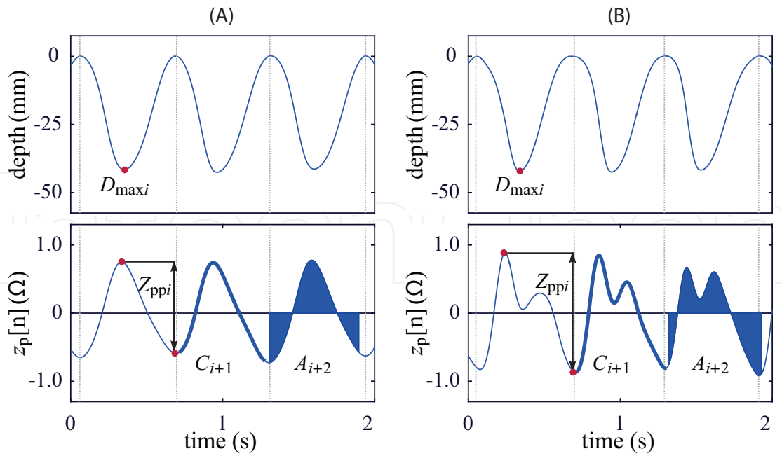
Figure 9. Two examples of the features extracted from the TI signal. The maximum depth is represented in the compression depth signal (top) and the TI features in the TI signal (bottom). Compression cycles are delimited by vertical dotted lines.
