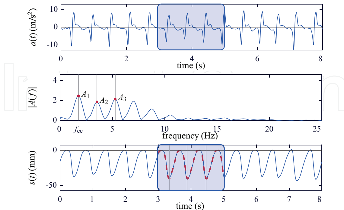
Figure 6. SAA method, based on the spectral analysis of the acceleration.
