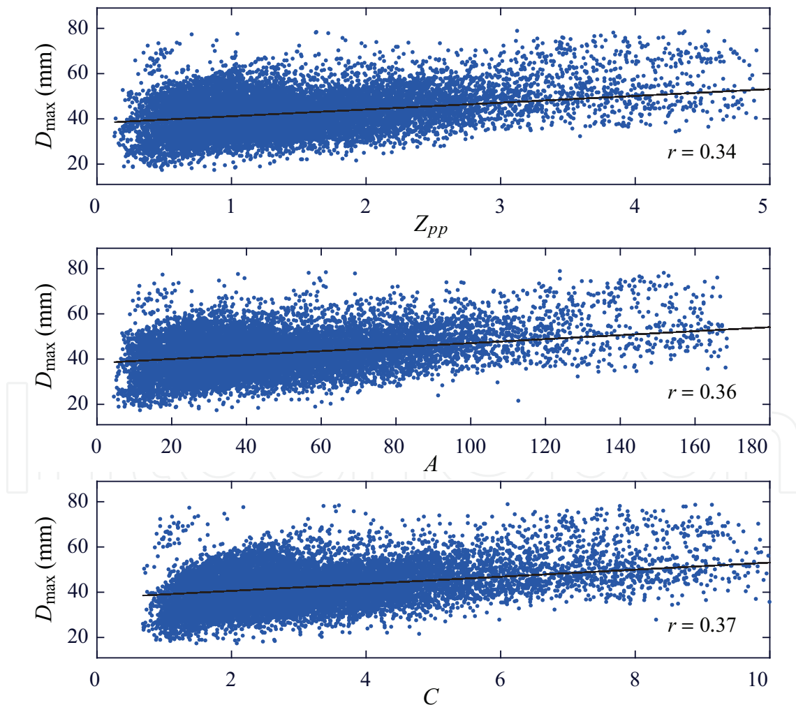
Figure 10. Scatterplots of D_{\max} with respect to TI features for the whole population. For each scatterplot, the fitted regression line and the value of r are depicted.
