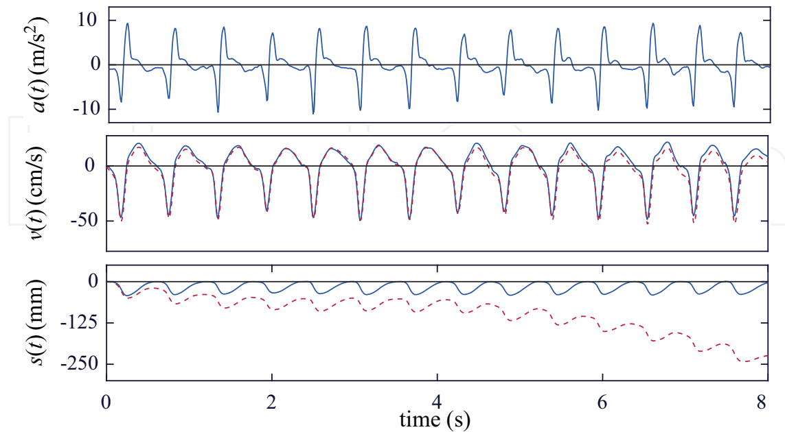
Figure 1. Integration errors in the displacement signal after the application of direct double integration to the acceleration signal.
