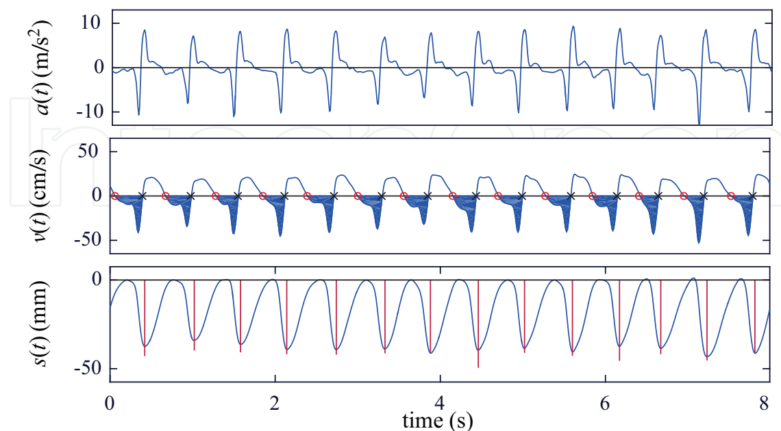
Figure 5. ZCV method, based on the analysis of velocity.
