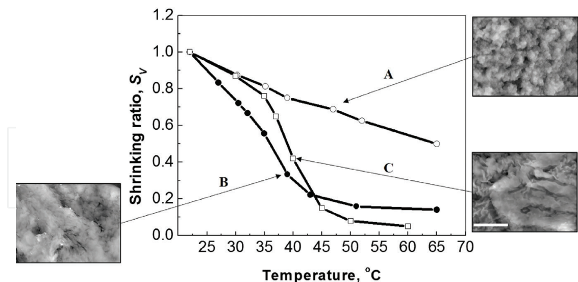
Figure 6. Shrinkage abilities S_V and SEM images of the microstructures of PNIPA hydrogels prepared by thermal polymerization in water (A) or DMSO (B), and by UV polymerization in water (C) (scale bar = 5 \mu\text{m} ).
