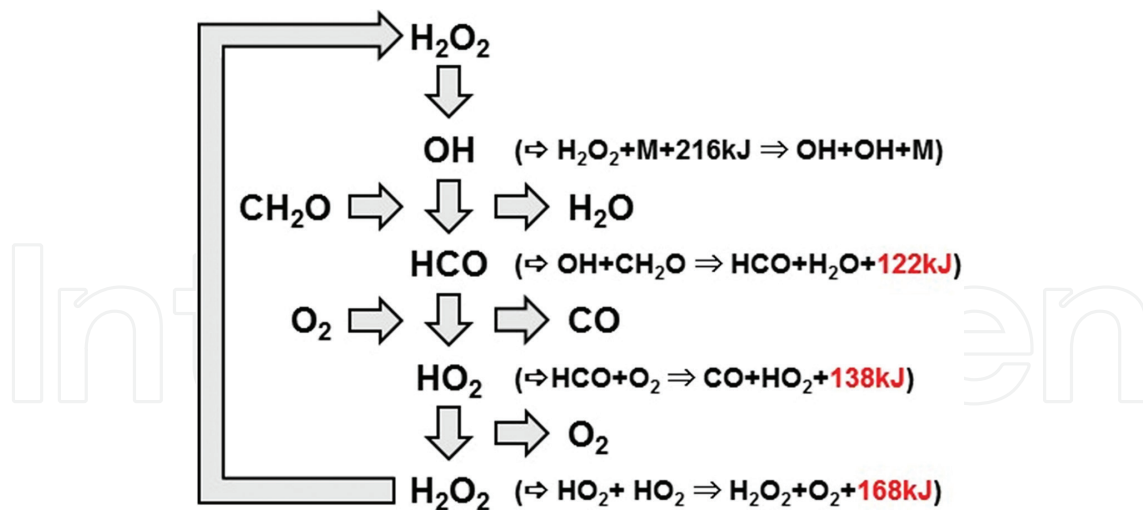
Figure 5. Schematic of H 2 O 2 reaction loop [24].
