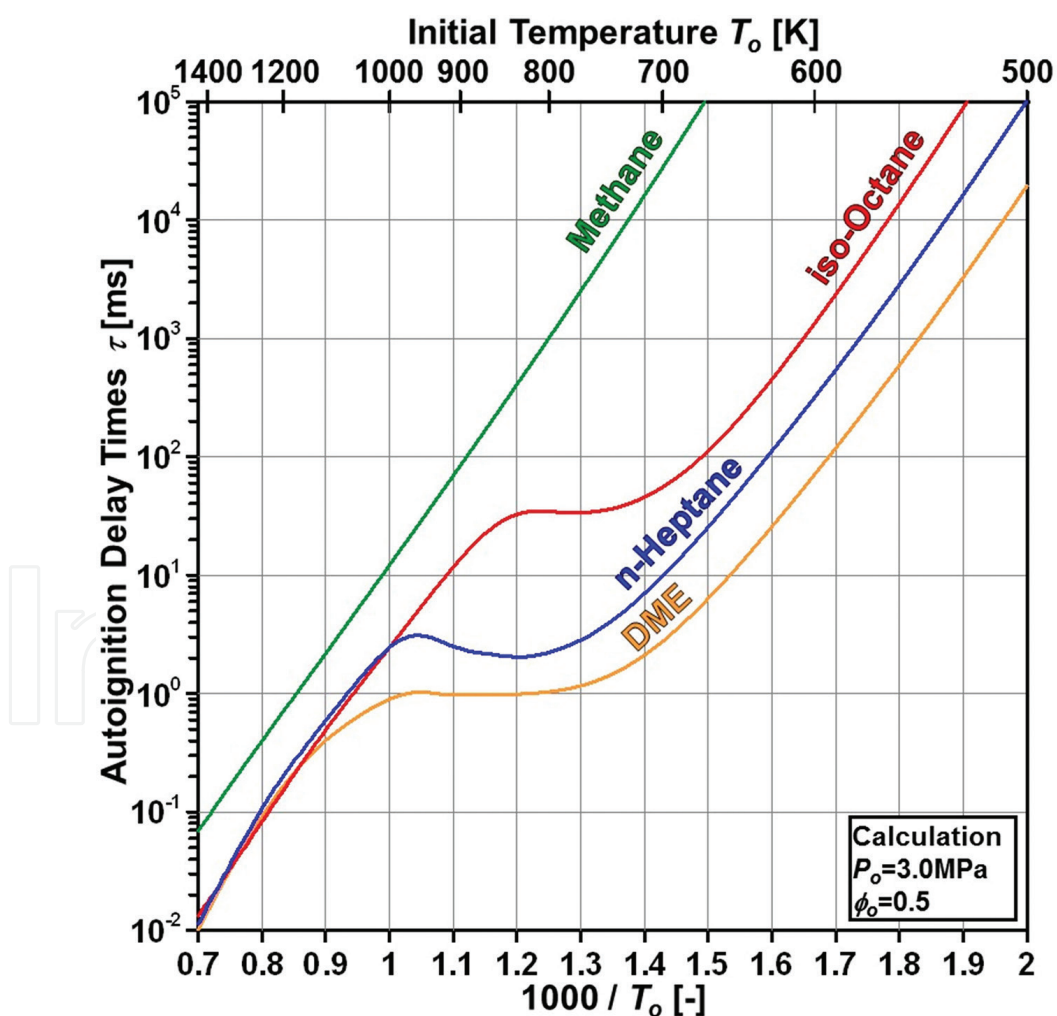
Figure 3. Comparison of autoignition delay times for methane, DME, n-heptane and iso-octane.
