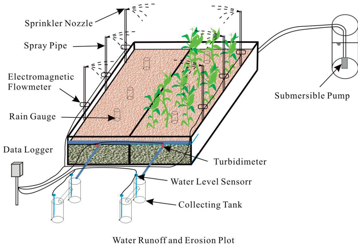
Figure 6. Schematic layout of water runoff and erosion plots.
