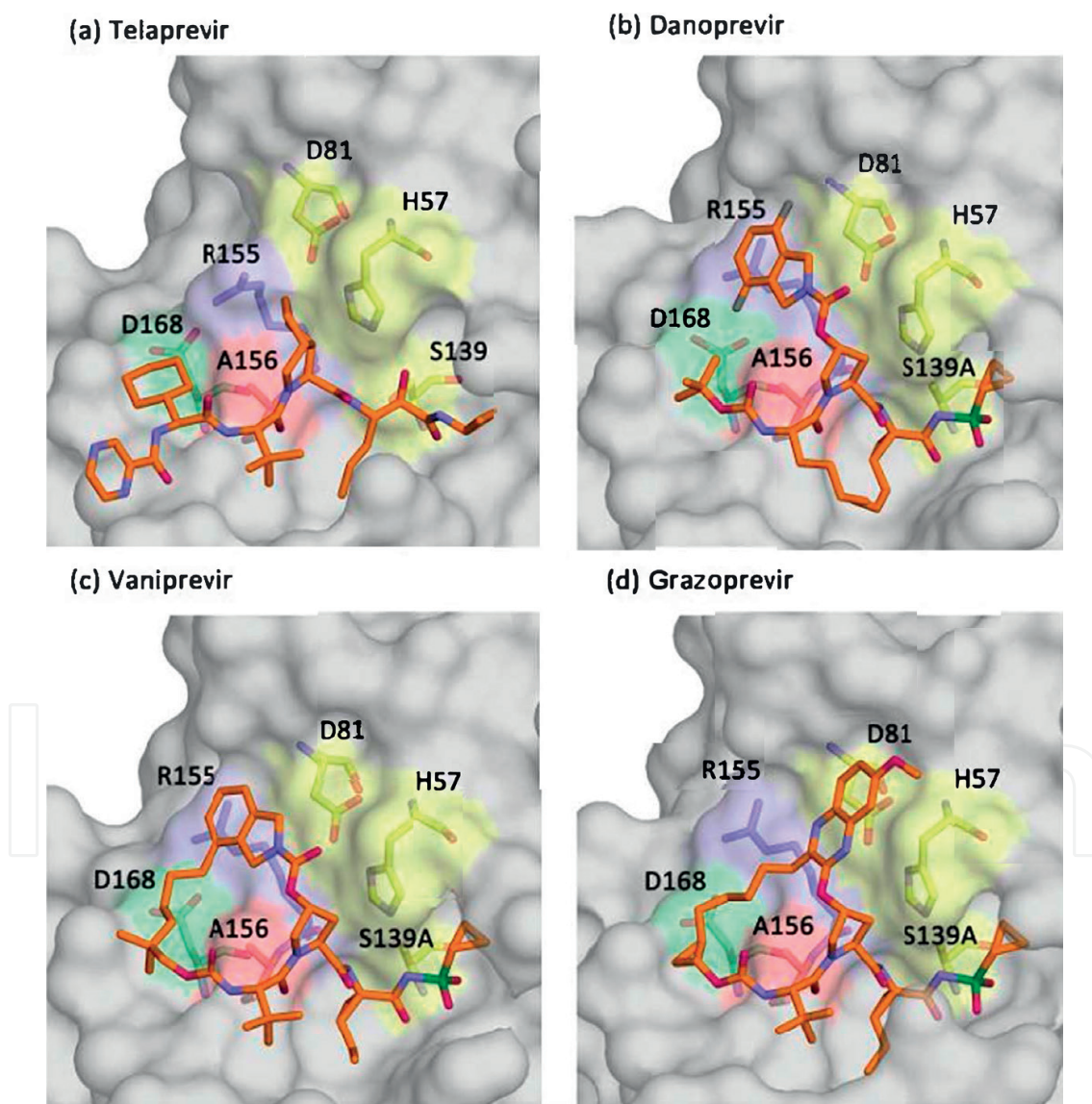
Figure 2. The binding conformations of telaprevir, danoprevir, vaniprevir, and grazoprevir. Surface representations of the wild-type protease in complex with (a) telaprevir, (b) danoprevir, (c) vaniprevir, and (d) grazoprevir. The catalytic triad consists of D81, H57, and S139A. The R155, A156, and D168 side chains are also labeled for each binding conformation. (Adapted from Romano et al. [5]).
