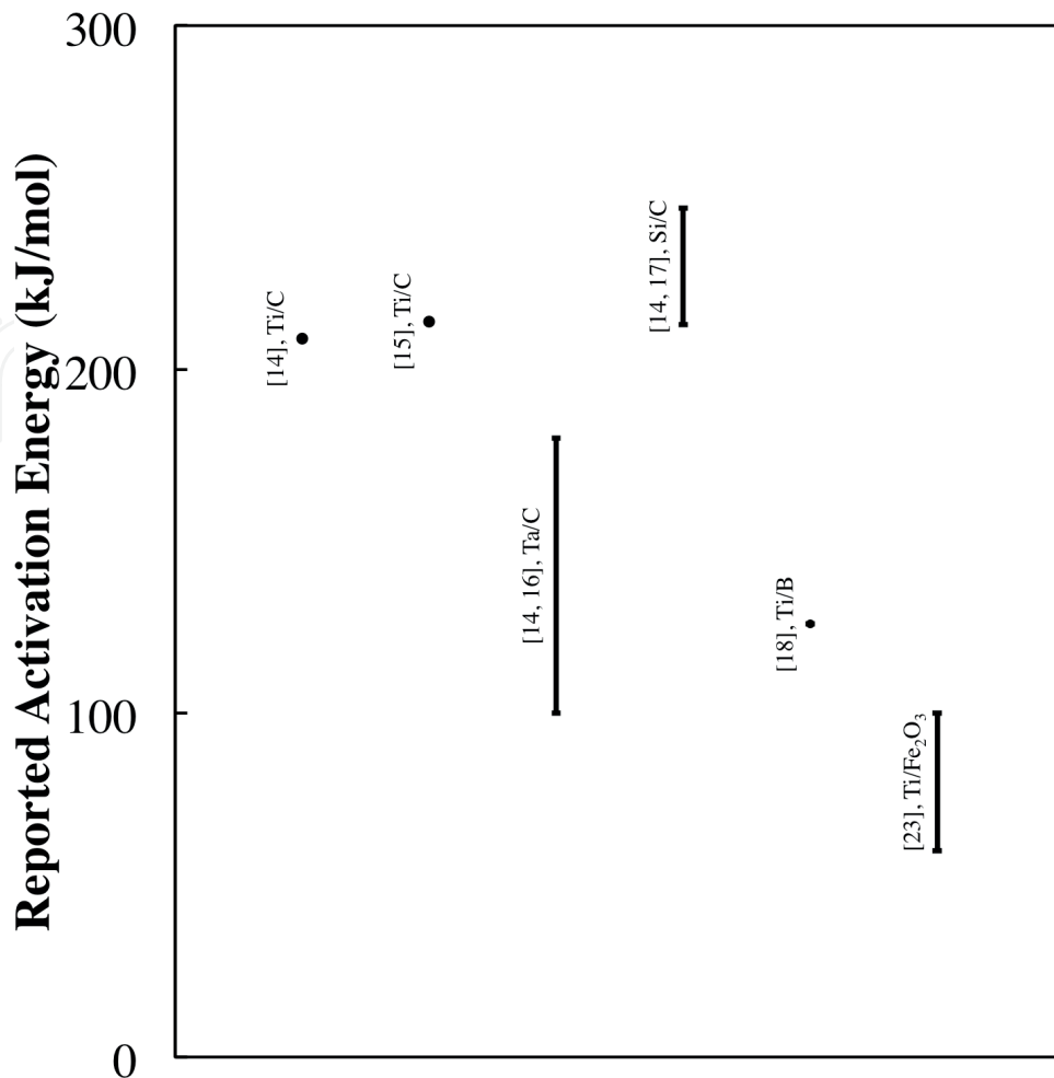
Figure 1. Summary of data collected using the electrothermal explosion technique.
