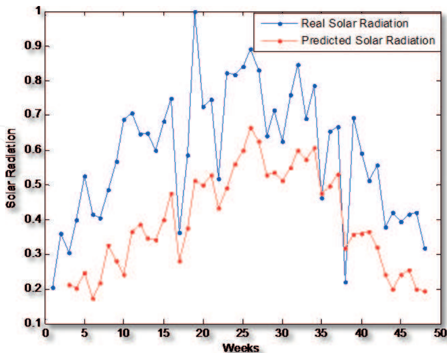
Figure 9. Solar radiation prediction using the static neural network.
