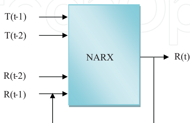
Figure 12. Neural architecture for the NARX model.
