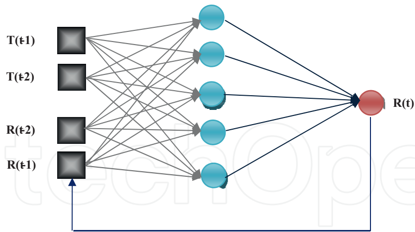
Figure 14. Optimal neural architecture for the NARX model.
