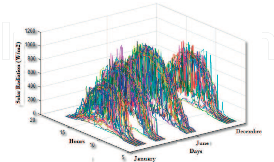
Figure 4. Solar radiation daily evolution during 2010.
