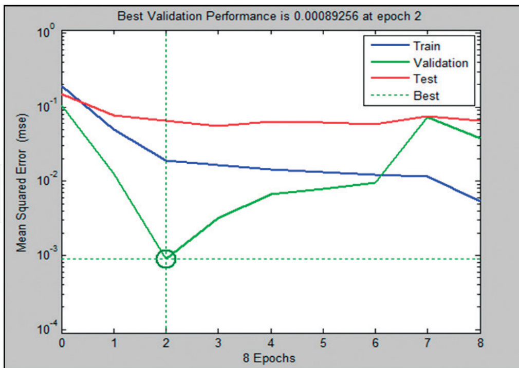
Figure 13. Learning, test and validation of NARX model.
