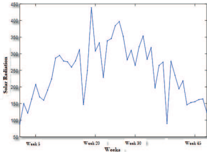
Figure 5. Weekly evolution of solar radiation during 2010.
