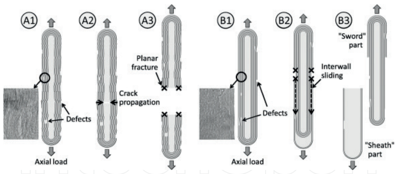
Figure 6. Schematic description of possible fracture mechanisms of MWCNTs annealed at different temperatures [53]. Shown are examples of (A1–A3) clean break -type failure and (B1–B3) sword-in-sheath -type failure.
