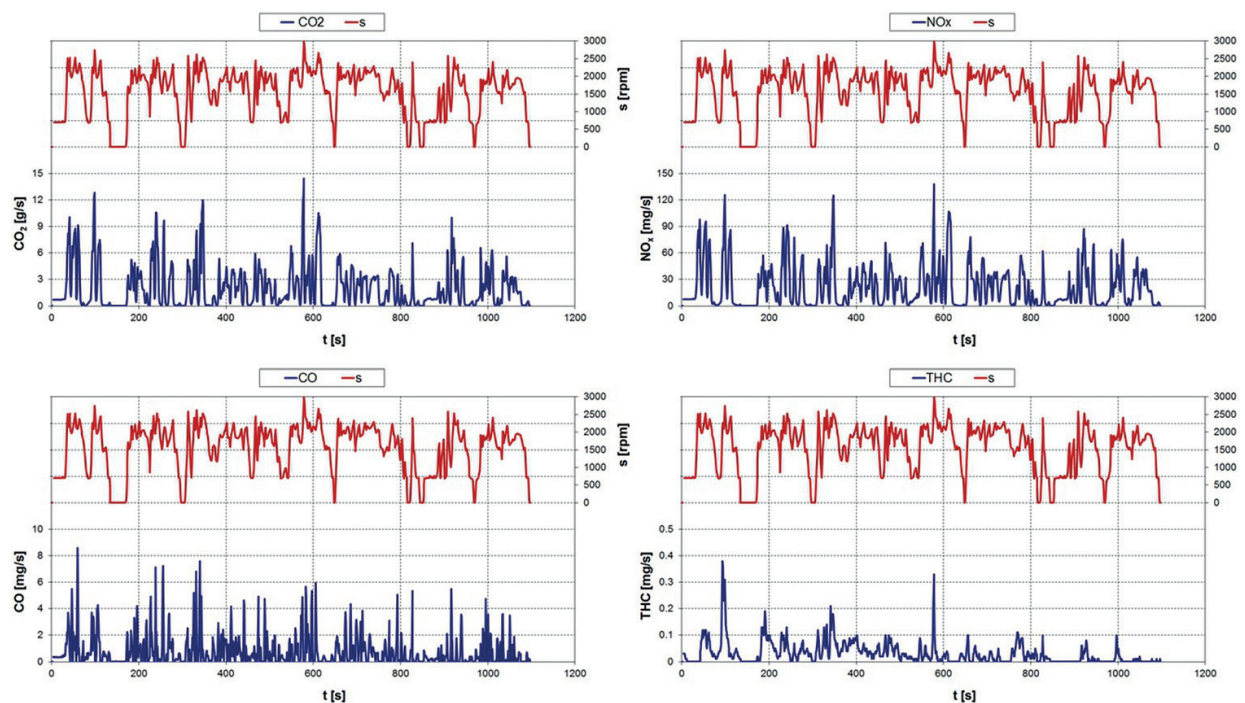
Figure 10. The courses of the emissions of CO_2 , NO_x , CO, and THC measured with the second-by-second resolution and engine speed of vehicle B during a drive with the start-stop system enabled.
