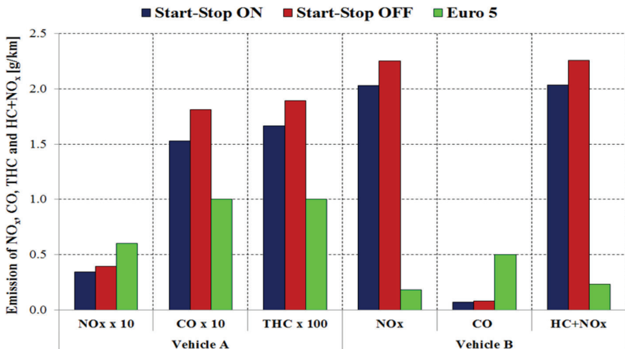
Figure 11. The obtained on-road emissions of \text{NO}_x , CO, THC, and HC + \text{NO}_x referred to the limits determined in the Euro 5 standard.
