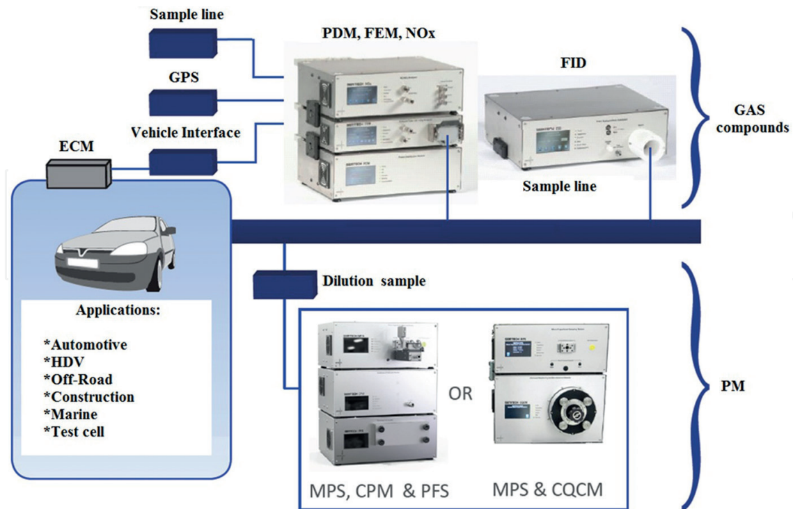
Figure 3. SEMTECH ECOSTAR analyzer for the measurement of gaseous exhaust components and particulate mass under actual conditions of operation [15].
