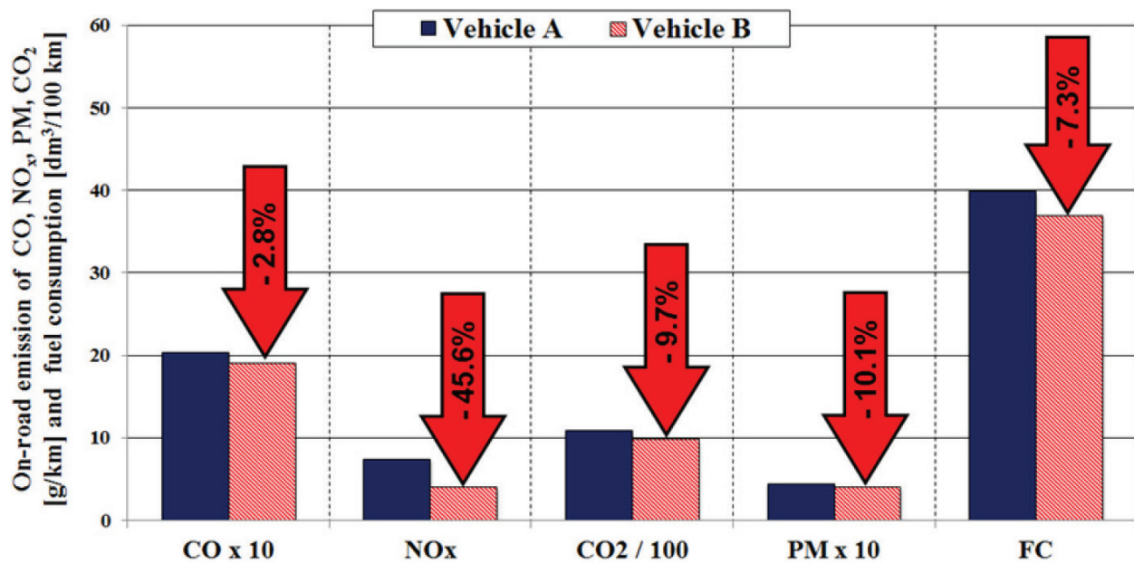
Figure 22. Comparison of the on-road emission of CO, NO x , CO 2 , PM and gas mileage of the tested vehicles.
