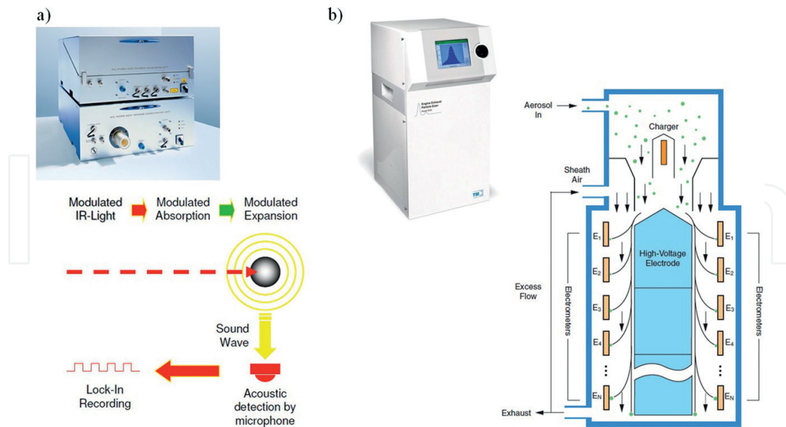
Figure 2. Equipment: (a) AVL MSS analyzers for the measurement of PM [13] and (b) TSI 3090 EEPS™ equipment for PM size distribution under actual conditions of operation [14].
