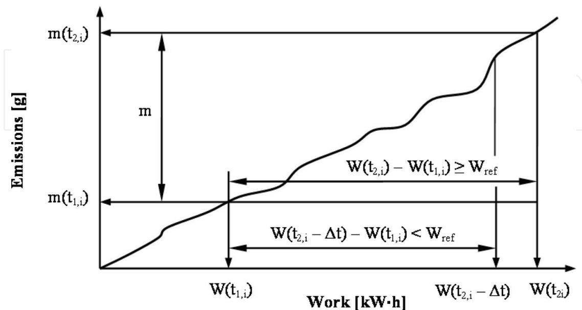
Figure 16. Determination of the measurement windows in the method based on reference work [28].
