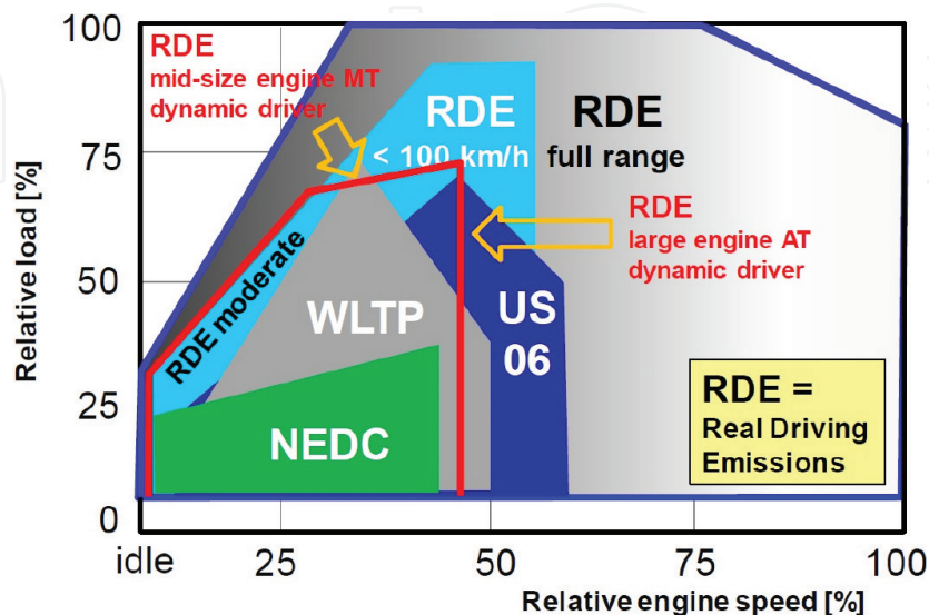
Figure 6. Engine parameters in different emission tests [22].
