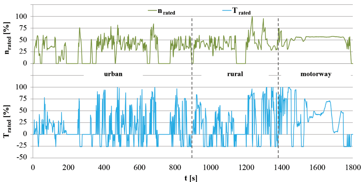
Figure 14. The engine torque and speed curves during the WHTC test [27].
