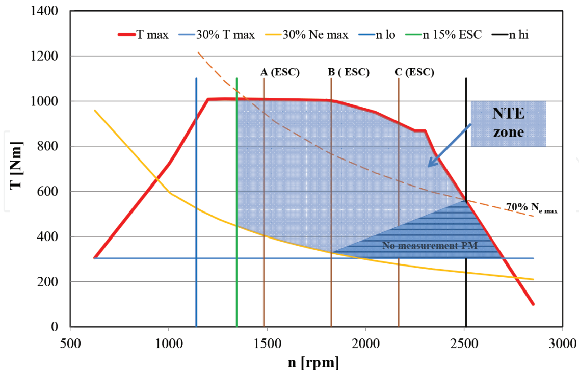
Figure 17. The NTE test area for the engine of a heavy-duty vehicle.
