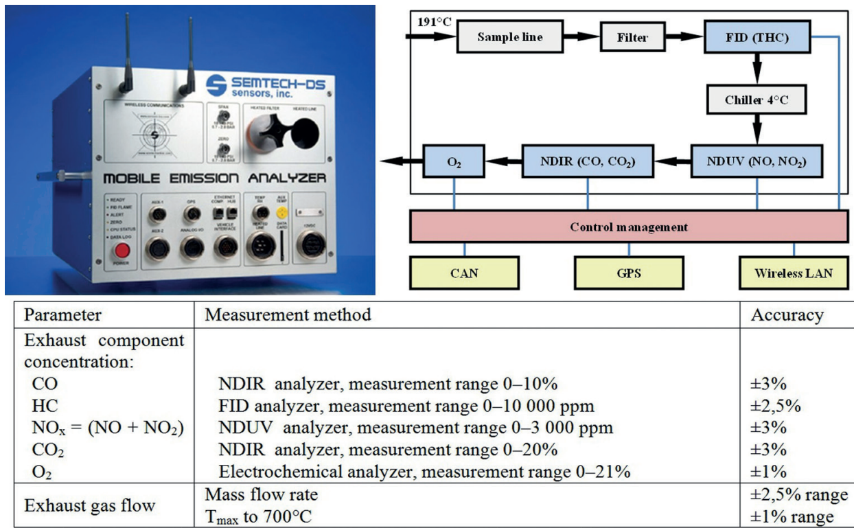
Figure 1. SEMTECH DS analyzer used for the measurement of exhaust gaseous components under actual conditions of operation [12].
