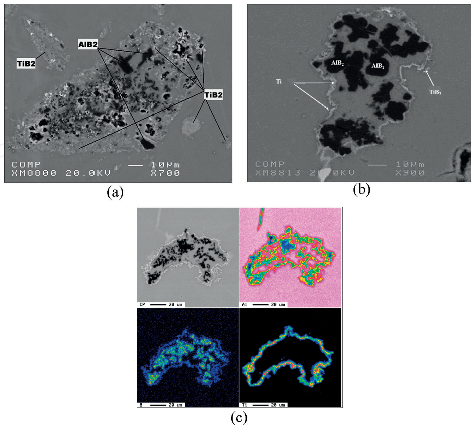
Figure 6. (a) Decomposition of Al-5%Ti-1%B master alloy, (b) backscattered electron image and (c) element distribution of Ti-B interaction in 1050 aluminum treated with 240 ppm B. Note the attraction of Ti ring toward the cluster of B-rich particles.
