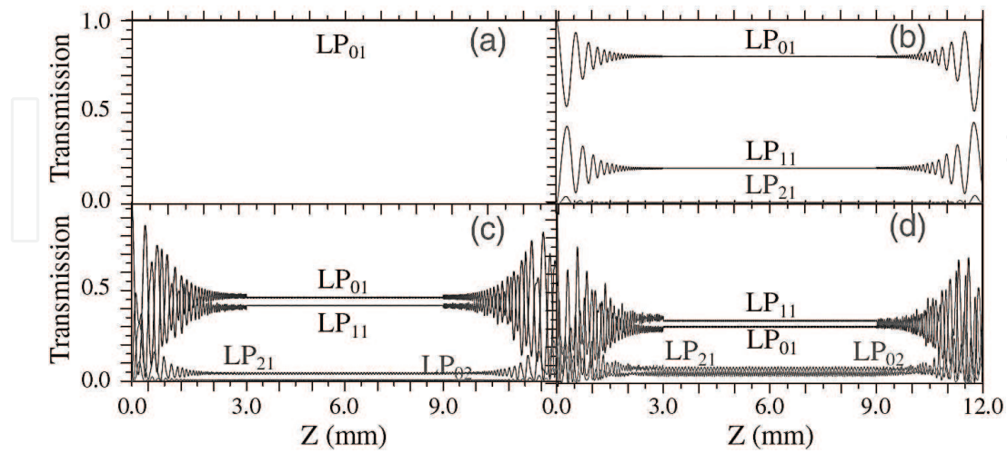
Figure 4. LP_{nm} local-mode power longitudinal evolution of the LBMT with d_0 = 3.7 \mu\text{m} and L_0 = 6 \text{ mm} under bending curvature 1/R being (a) 0, (b) 0.2, (c) 0.445, and (d) 0.526 \text{ mm}^{-1} at \lambda = 1.555 \mu\text{m} .
