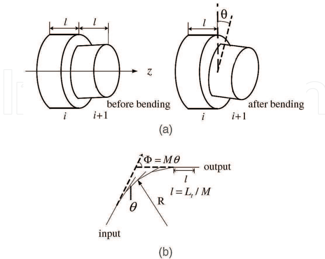
Figure 3. (a) Two adjacent sections of a fiber before and after bending. (b) Geometry used for the theoretical analysis of the bending effect on the fiber taper [15].
