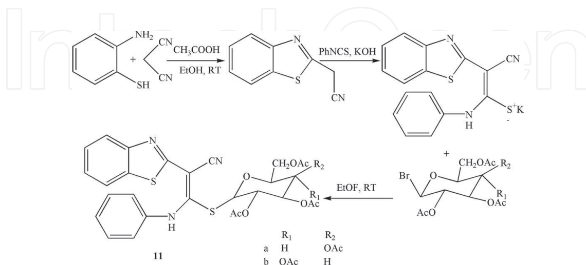
Figure 11. Synthesis of thioxoimidazolidin and benzothiazole derivatives.
