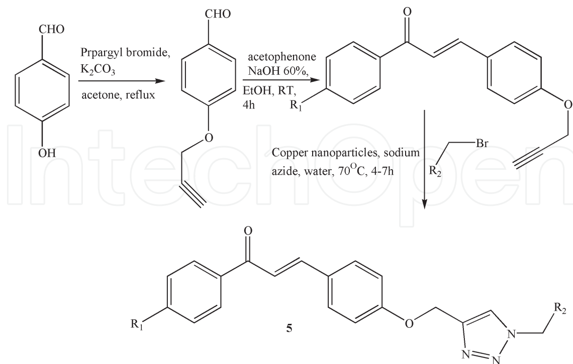
Figure 5. Synthesis of chalcone derivatives.
