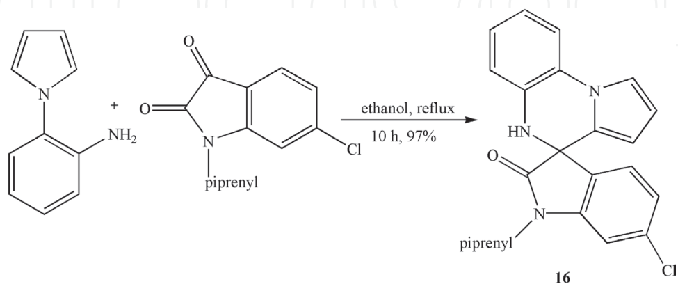
Figure 16. Synthesis of spiro[indoline-3,4'-pyrrolo(1,2-a)quinoxalin].
