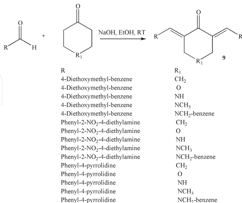
Figure 9. Synthesis of \alpha,\beta -unsaturated carbonyl-based compounds.
