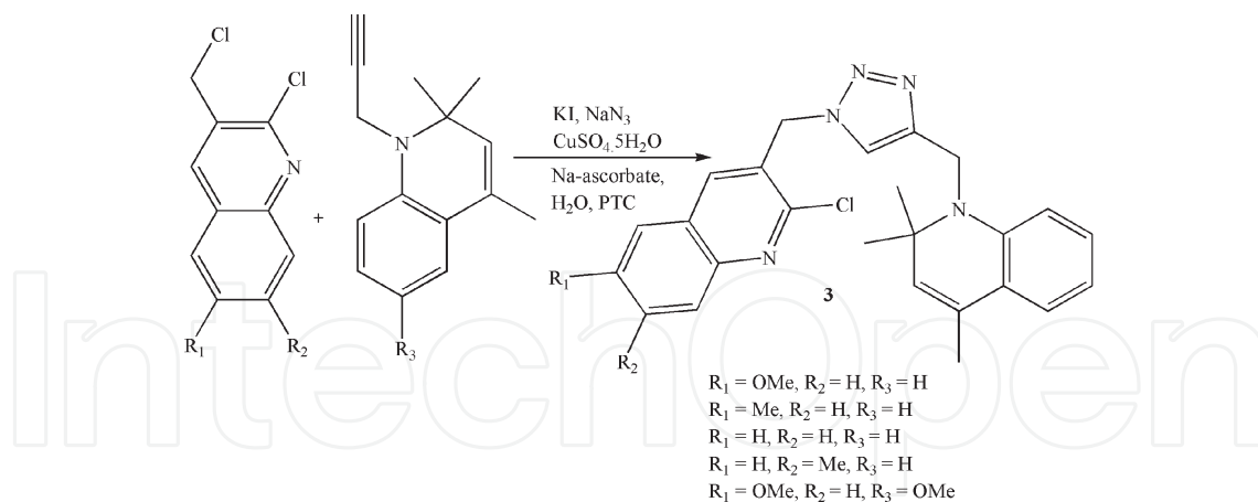
Figure 3. Synthesis of polyazaheterocycles.
