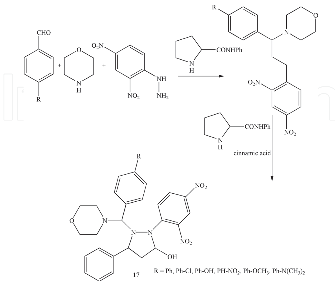
Figure 17. Synthesis of morpholine-connected pyrazolidine.
