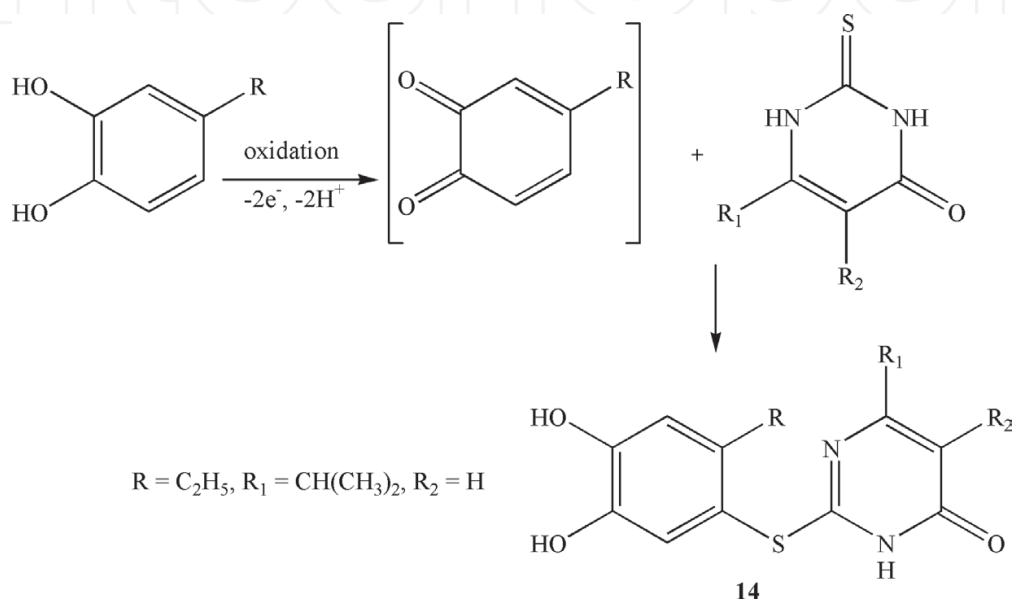
Figure 14. Synthesis of pyrimidobenzothiazoles.
