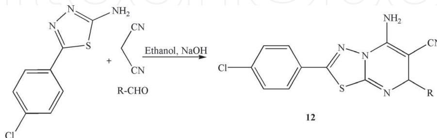
Figure 12. Synthesis of pyrimidine-6-carbonitrile derivatives.
