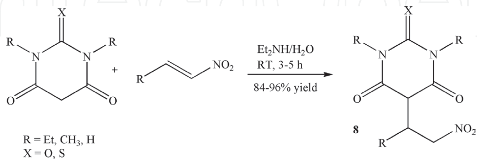
Figure 8. Synthesis of quinoline cycloheximide.
