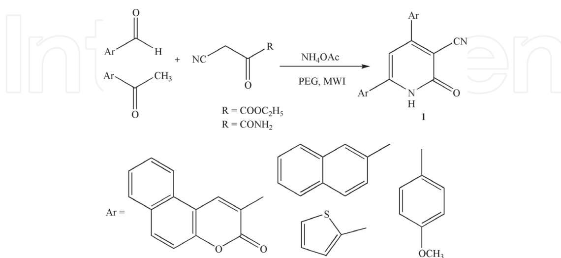
Figure 1. 3-cyano pyridine derivatives.
