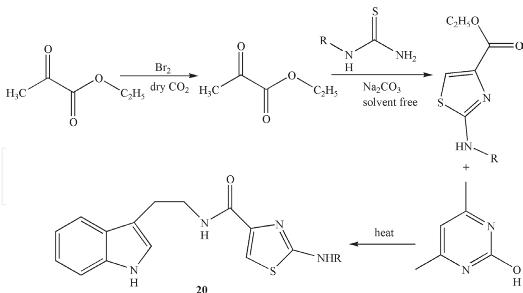
Figure 20. Synthesis of bacillamide analogues.
