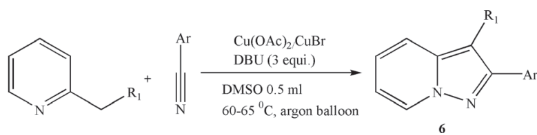
Figure 6. Synthesis of pyridine derivatives.
