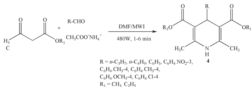
Figure 4. Synthesis of carboethoxy/carbomethoxy derivatives.
