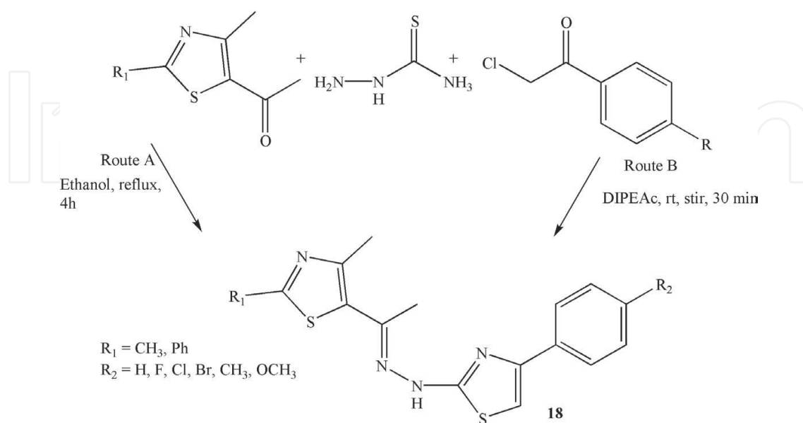
Figure 18. Synthesis of bithiazolyl hydrazones.
