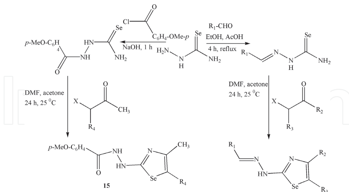
Figure 15. Synthesis of 1,3-selenazole derivatives.
