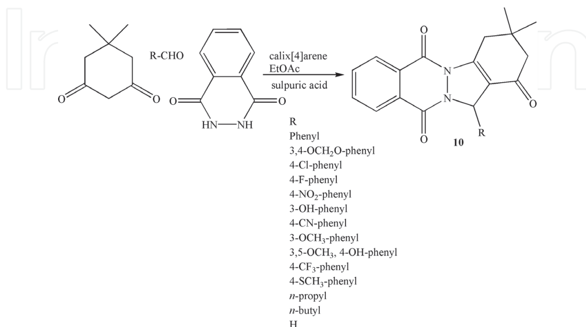
Figure 10. Synthesis of phthalazine-trione derivatives.
