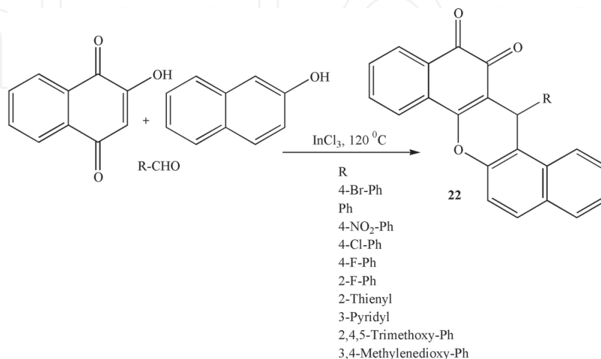
Figure 22. Synthesis of o -quinonic adducts.
