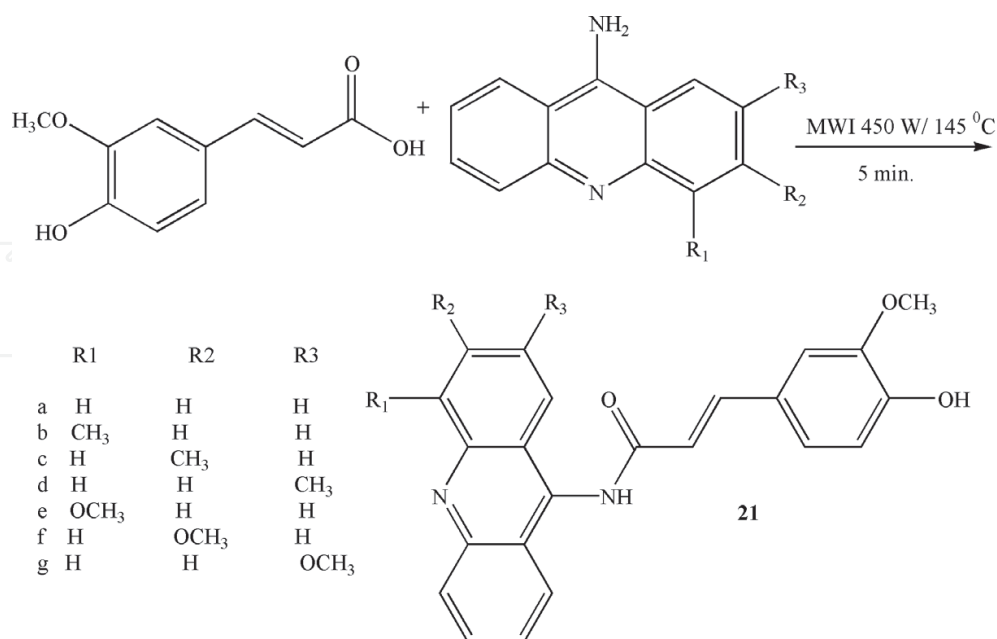
Figure 21. Synthesis of ferulic acid derivatives.
