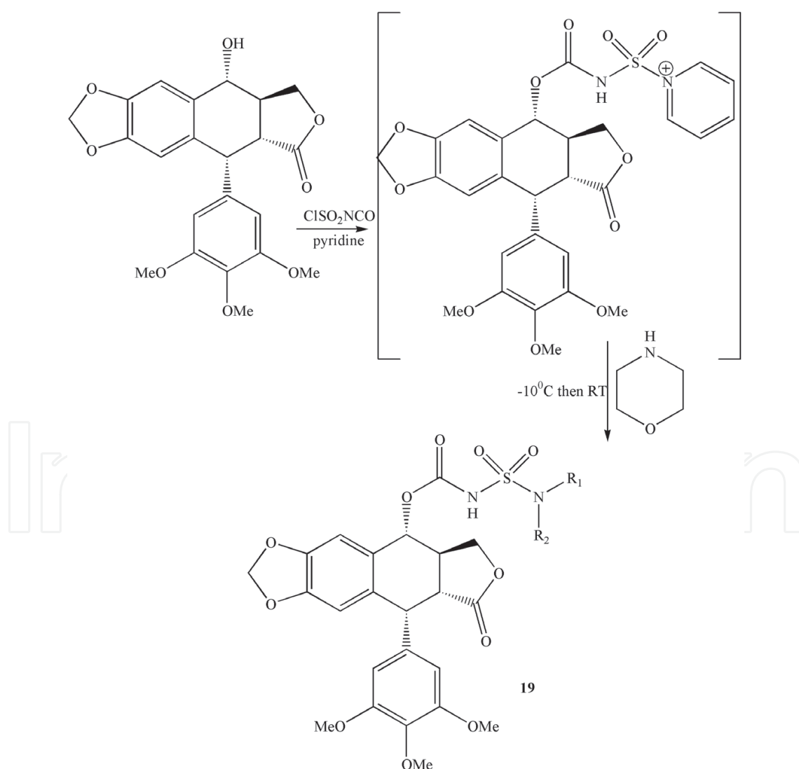
Figure 19. Synthesis of N-(aminosulfonyl)-4-podophyllotoxin carbamates.
