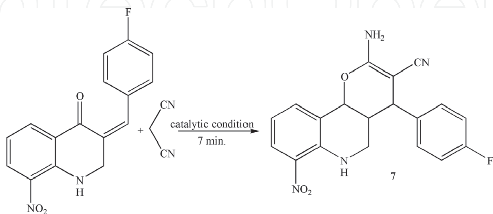
Figure 7. Synthesis of quinoline analogues.
