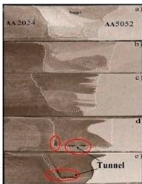
Figure 2. Cross sectional macrostructures of welded samples.
