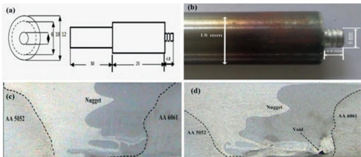
Figure 10. Dimensions of cylindrical threaded tool pin and cross sectional macrostructures of welded samples.
