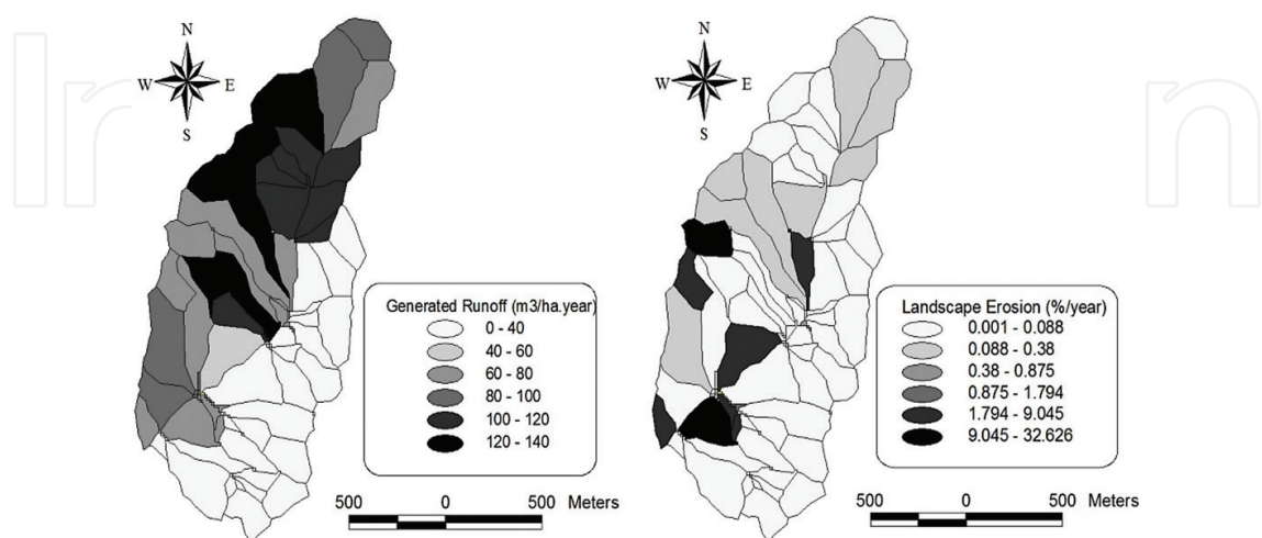
Figure 14. Average simulated runoff and erosion rates, generated in each cell and subcatchment, by AnnAGNPS model (period 2003–2005).
