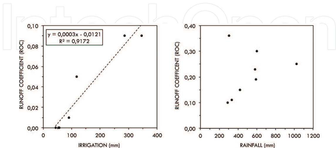
Figure 11. Runoff coefficient ( ROC ) in irrigation and rainfed seasons evaluated in the study catchment.
