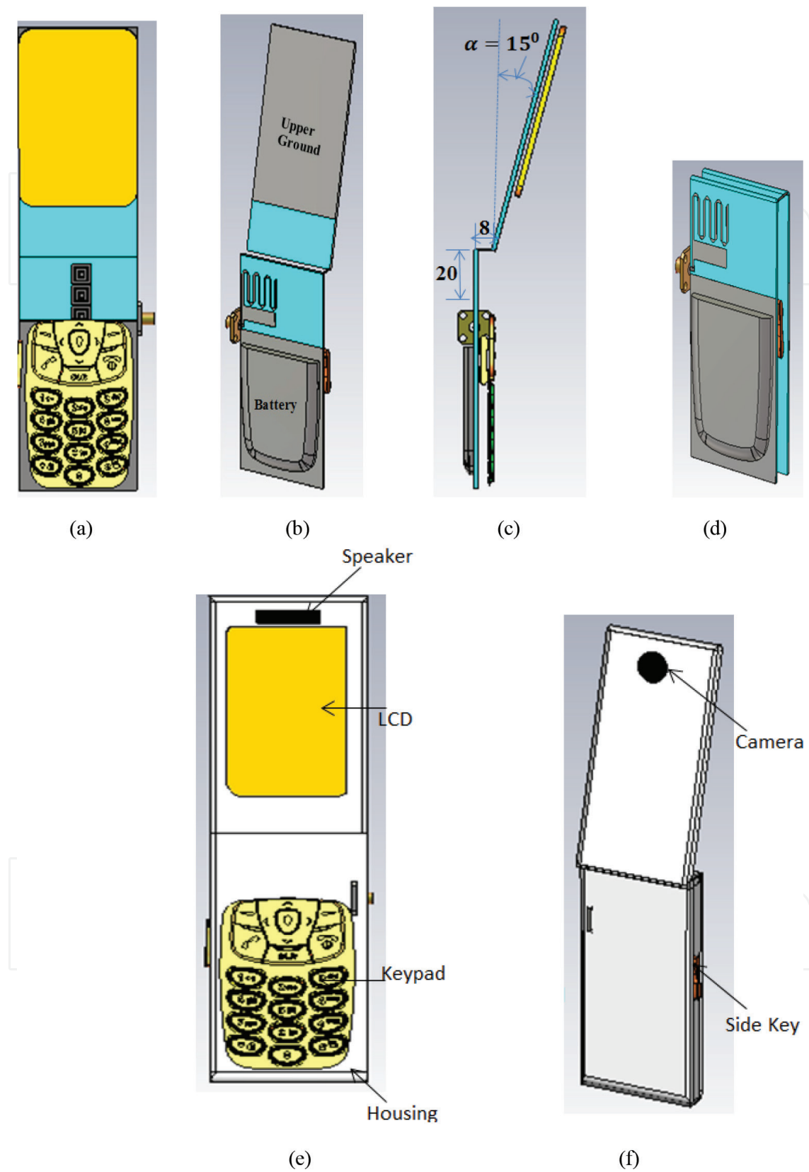
Figure 13. Geometry of the clamshell mobile. (a) Front view of clamshell without packaging. (b) Back view of clamshell without packaging. (c) Side view of clamshell without packaging. (d) Closed mode of clamshell without packaging. (e) Front view of clamshell with packaging. (f) Back view of clamshell with packaging.
