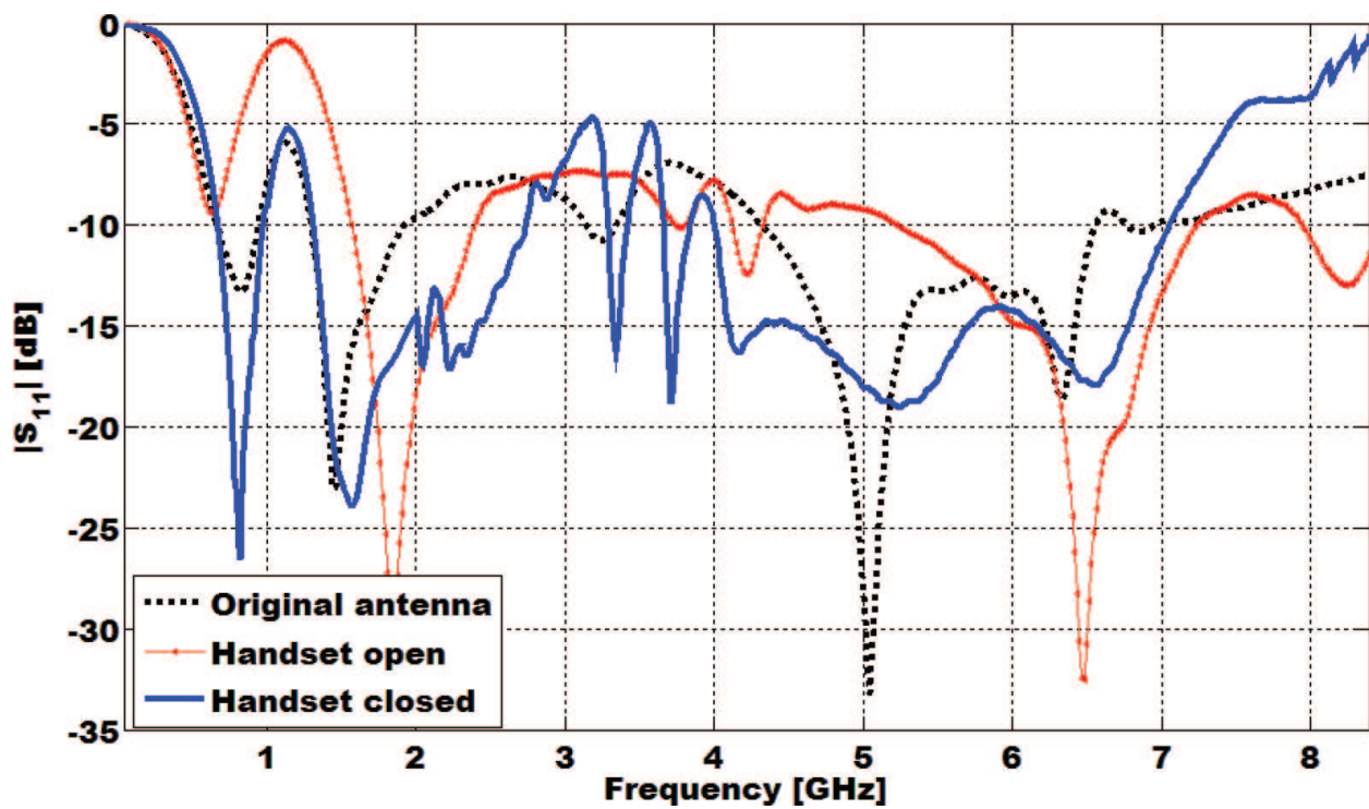
Figure 15. The simulated return loss of original antenna and antenna in handset.
