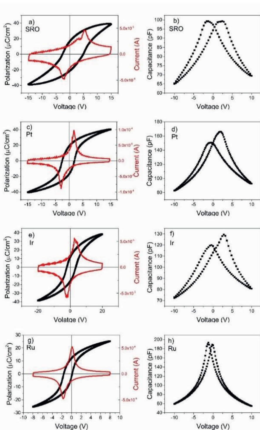
Figure 8. Hysteresis loops and capacitance-voltage characteristics obtained for different top electrodes: (a,b) for SRO, (c,d) for Pt, (e,f) for Ir and (g,h) for Ru, respectively.
