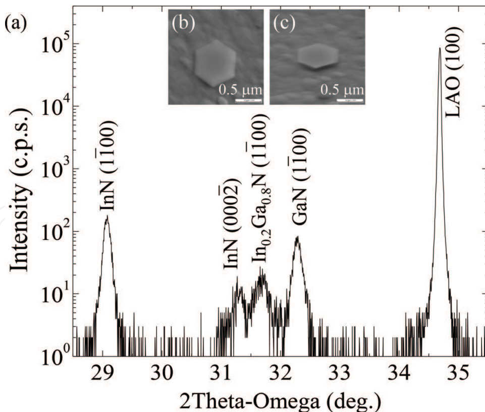
Figure 5. (a) The X-ray 2Theta-Omega scan of the sample. (b) The top-view SEM image of InN hexagonal thin disk, the scale bar is 0.5 μm. (c) The tilt-view SEM image of InN hexagonal thin disk, the scale bar is 0.5 μm.
