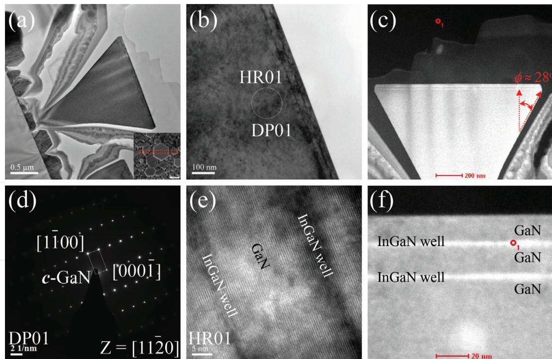
Figure 10. TEM analyses of the InGaN/GaN QW microdisk: (a) and (b) show the bright field images with [1\bar{1}\bar{2}0]_{\text{GaN}} // [001]_{\text{LAO}} zone axis, the scale bars are 0.5 and 100 nm, respectively. (c) The STEM image taken at the top area of InGaN/GaN QW, the scale bar is 200 nm. The selective area diffraction patterns taken at the points shown in (b) are presented in (d), the scale bar is 2 (1/nm). The high-resolution TEM images taken at the point shown in (b) are presented in (e), the scale bars are 2 nm. (f) The enlarged STEM image of InGaN/GaN QW (the scale bar is 20 nm).
