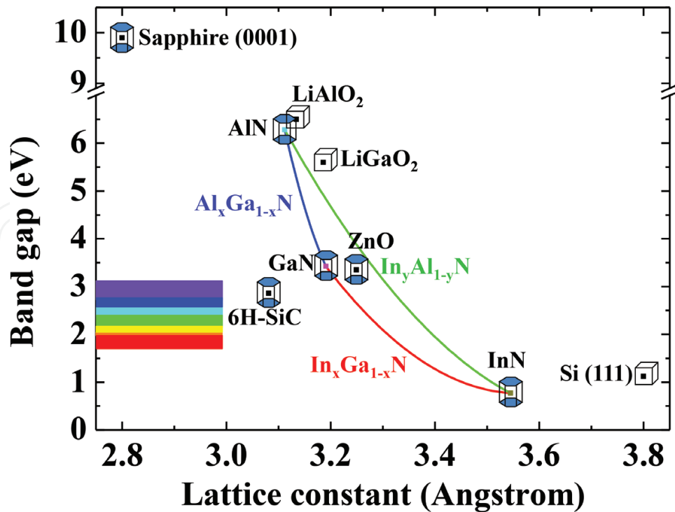
Figure 1. The diagram shows band-gap energies of III-nitrides with bowing parameters versus lattice constants. The substrate materials were also presented.
