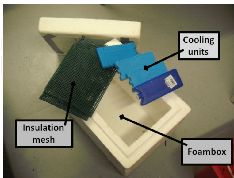
Figure 4. A simple and cost-efficient method for transporting crayfish on board and on land [10] with explanation on different parts inside the cooling box (an additional large plastic bag needed for protection of crayfish).
