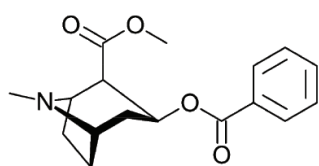
Cocaine
