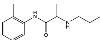
Prilocaine
