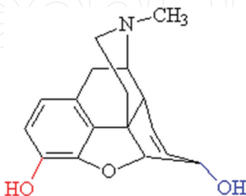
Figure 4. Morphine structure, replacing the —OH group shown in red with —OCH 3 , produces codeine where heroin derives from replacing both the red and blue —OH groups with OCOCH 3 .
