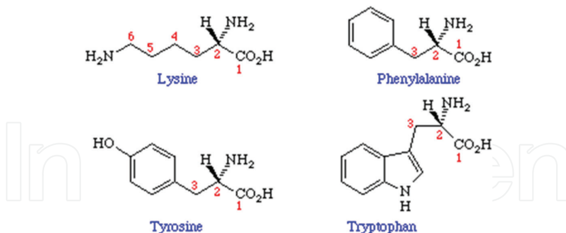
Figure 1. The amino acids used for alkaloid biosynthesis.
