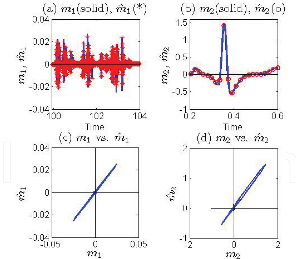
Figure 2. Responses of Rossler system: (a) m_1 and \hat{m}_1 ; (b) m_2 and \hat{m}_2 ; (c) m_1 vs. \hat{m}_1 ; and (d) m_2 vs. \hat{m}_2 . Figures 2(c) and 2(d) indicate negligible estimation error \hat{m}_1 = m_1 - \hat{m}_1 and small \hat{m}_2 = m_2 - \hat{m}_2 , respectively.
