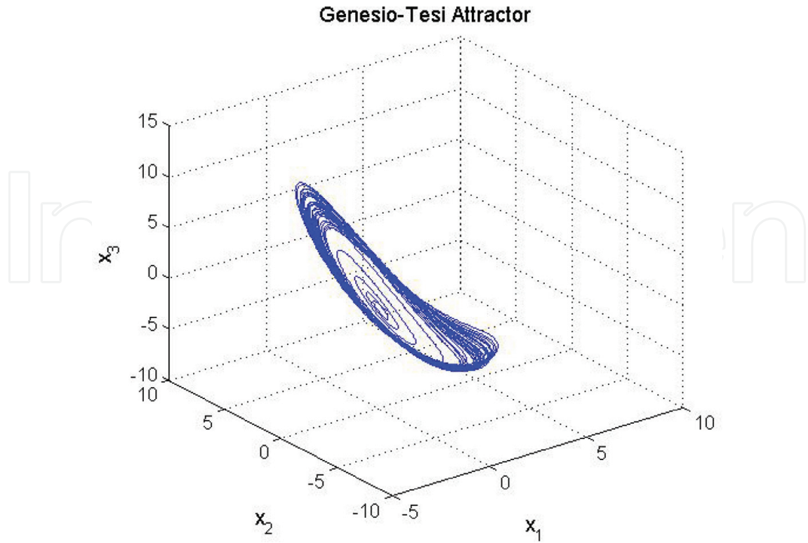
Figure 5. Genesisio-Tesi attractor obtained by using (46).
