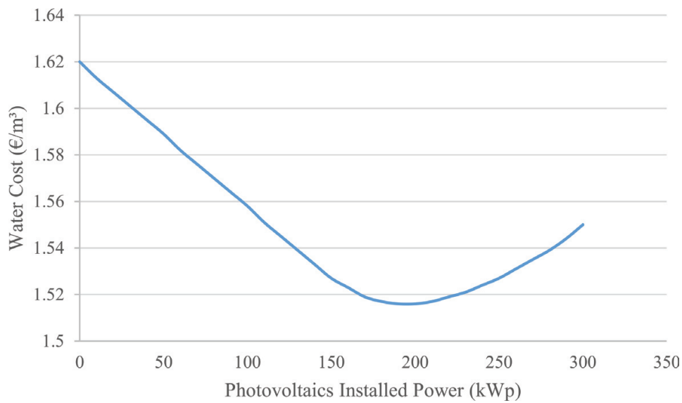
Figure 13. Water cost versus photovoltaic install power for Patmos.
