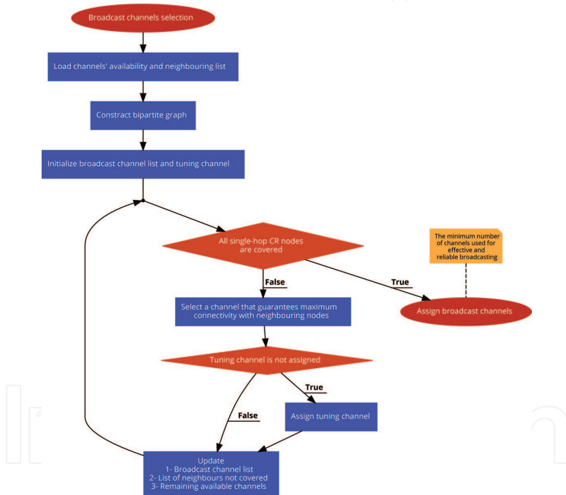
Figure 6. Flowchart for OBA.
