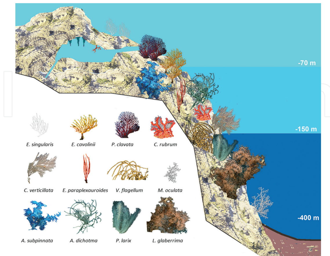
Figure 2. Zonation of the megabenthic assemblages. The figure presents the distribution of the most conspicuous and abundant components of the megafauna dwelling at about 50–500 m depth.
