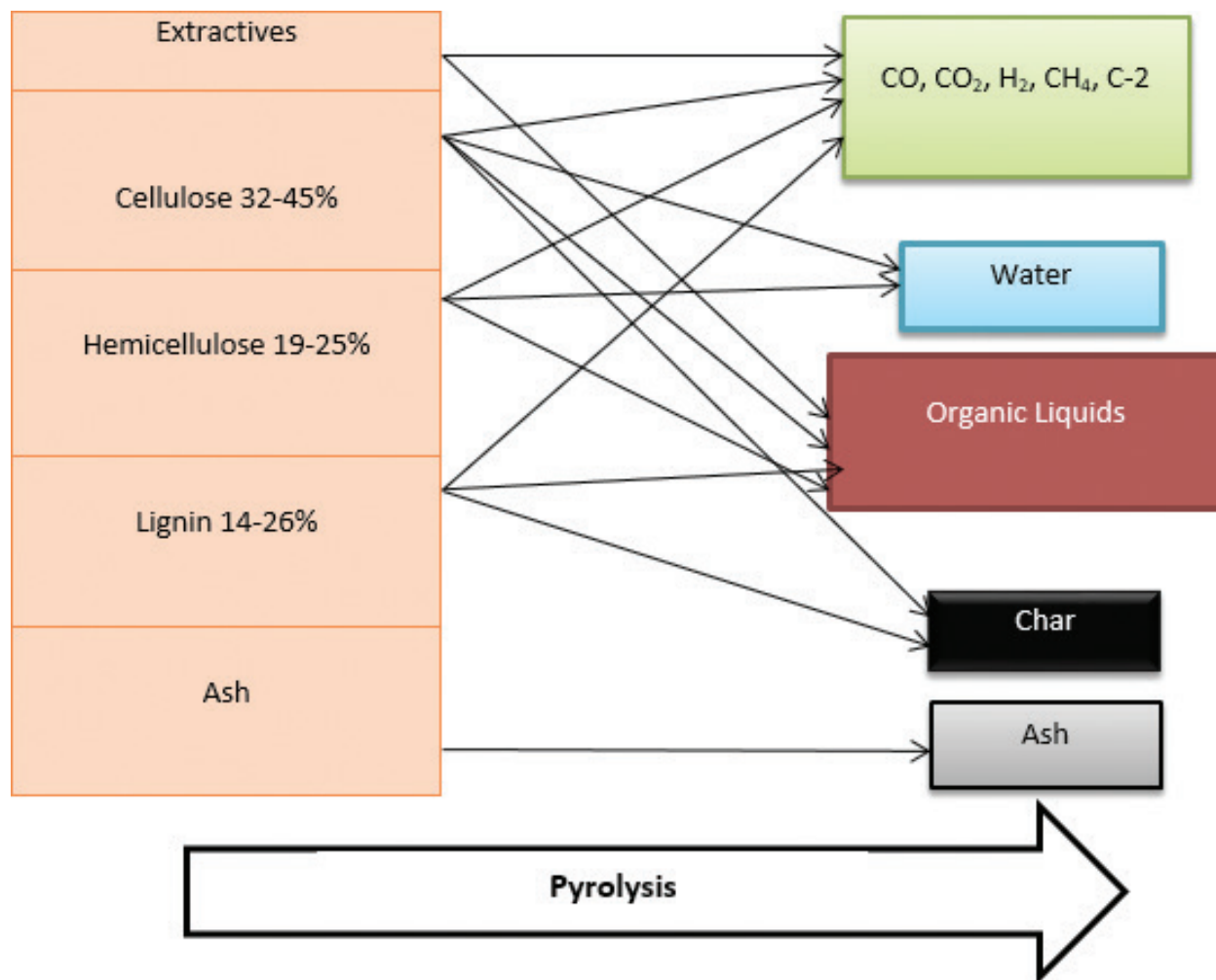
Figure 5. Product distribution during pyrolysis [29].
