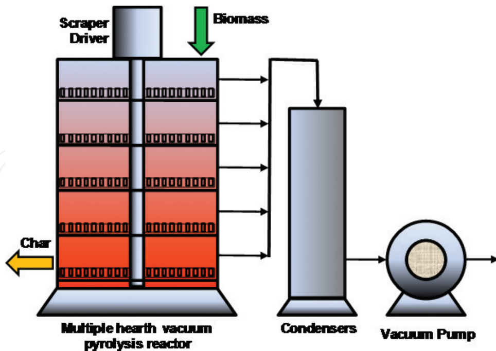
Figure 9. Vacuum reactor [83].
