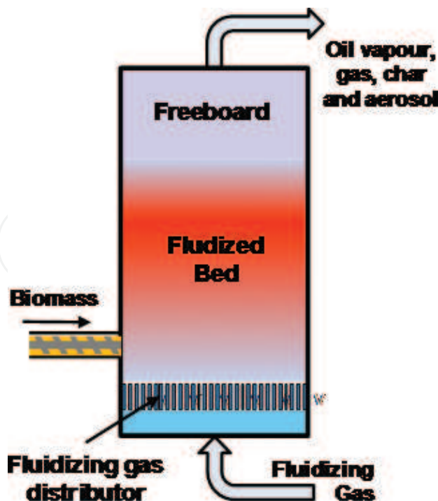
Figure 7. Bubbling fluidized bed reactor [80].
