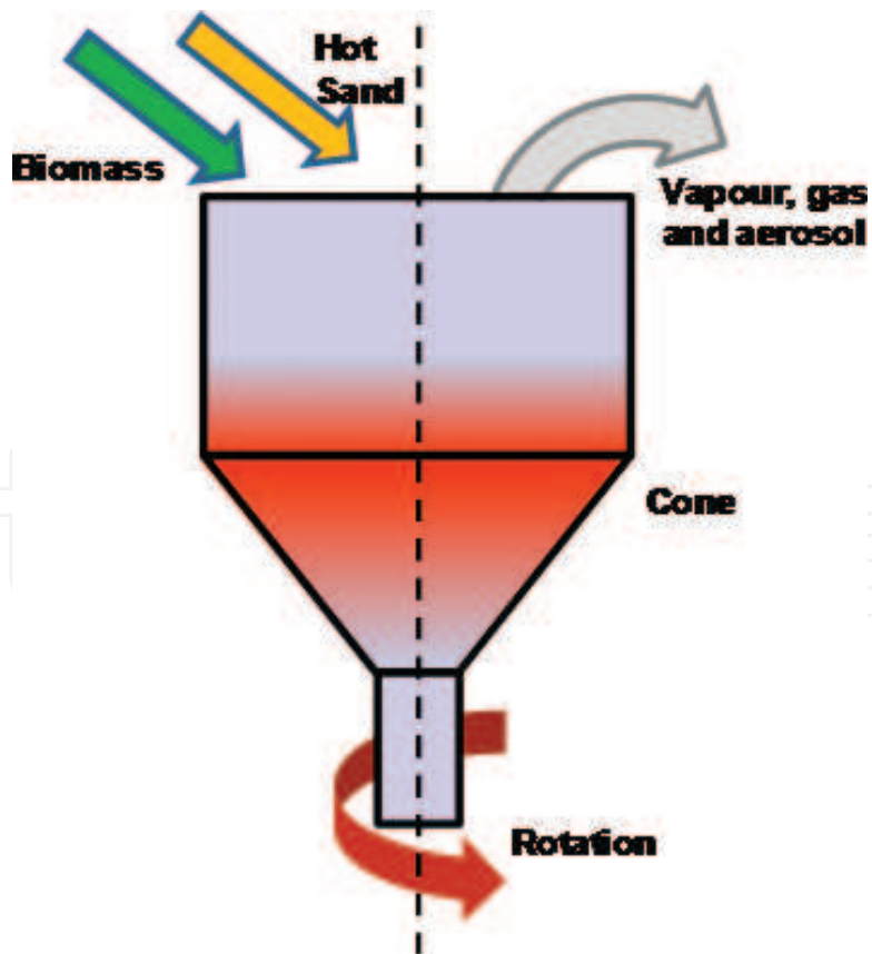
Figure 10. Rotating cone reactor [74].
