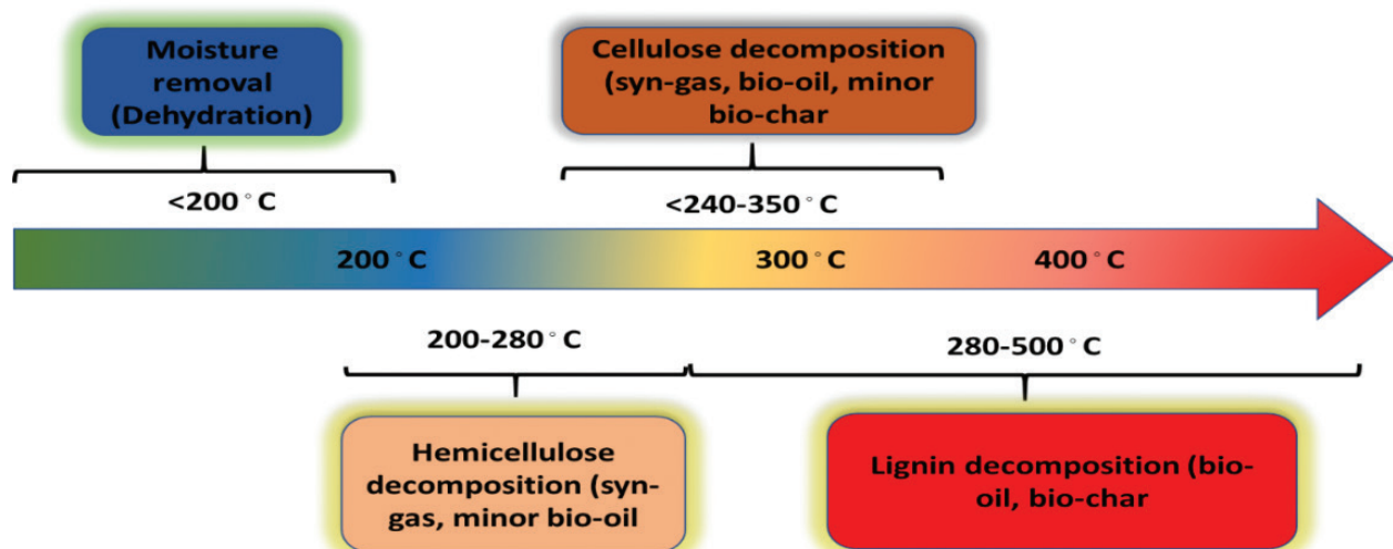
Figure 3. Decomposition behaviour of biomass constituents at different temperature [19].
