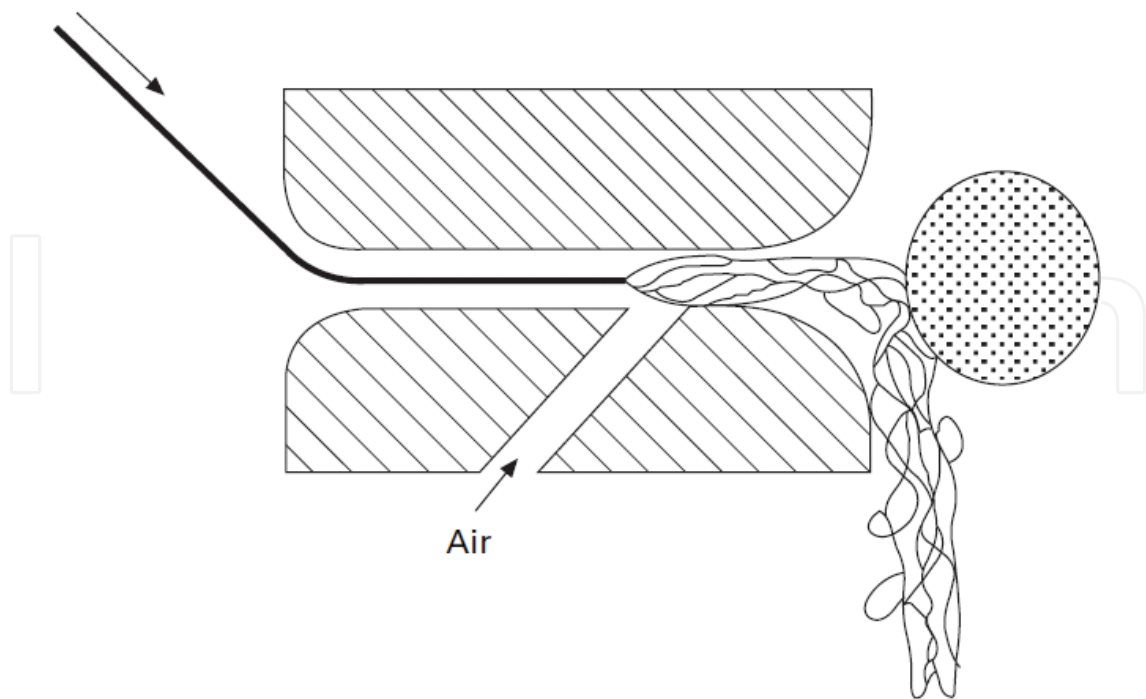
Figure 5. Air-jet yarn texturing [25].
