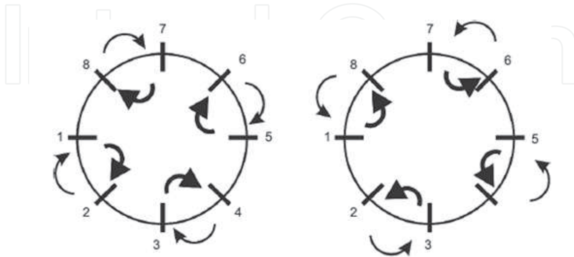
Figure 12. Sequence for tubular braiding [29].
