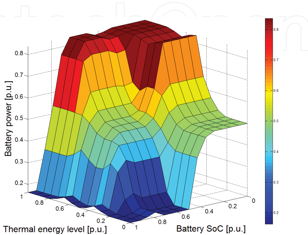
Figure 6. Response surface for the fuzzy logic supervisor.
